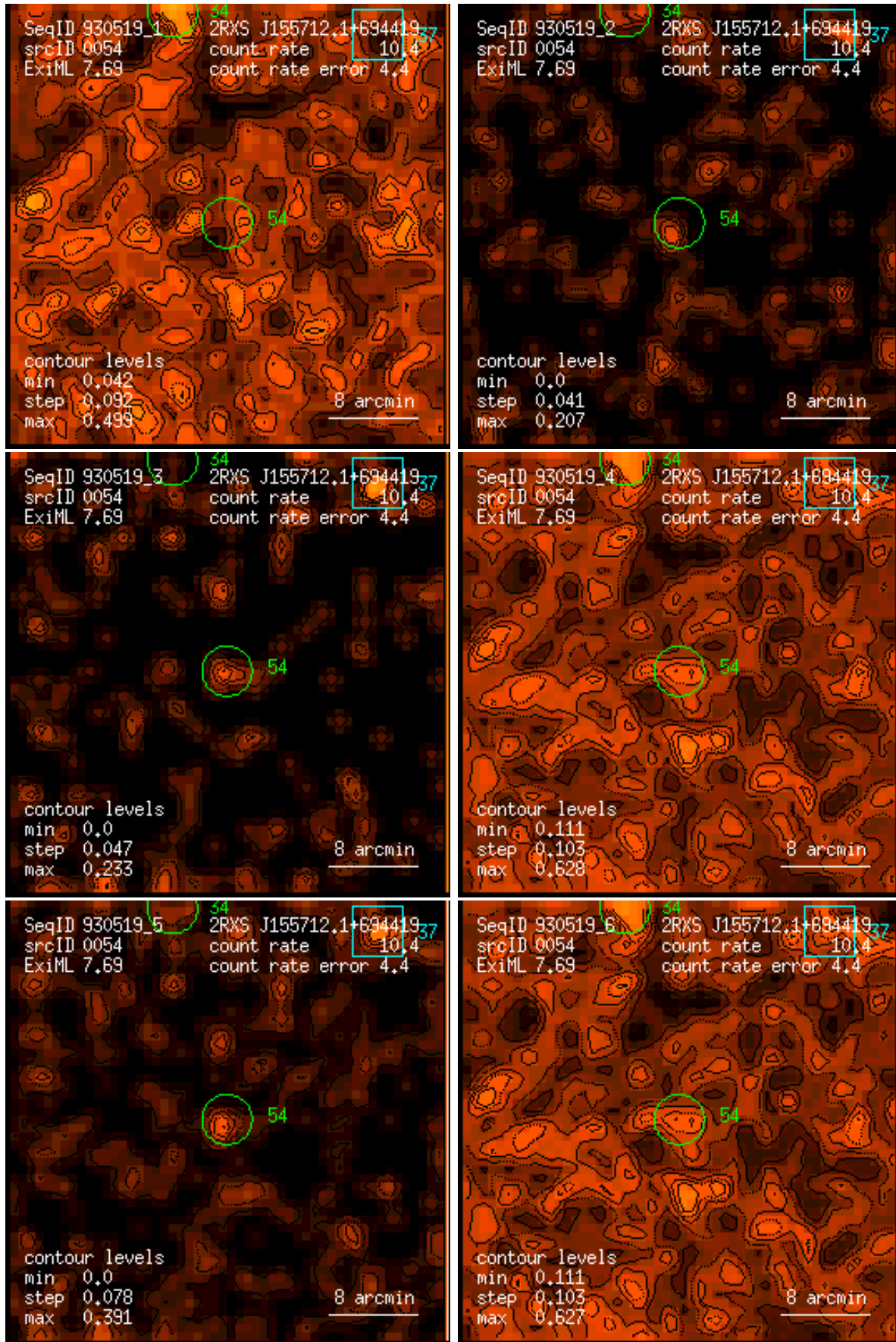
Figure 54: RASS 930519: detection 0054: band rate images, Gaussian filter: (1) PSPC channels 11 – 41, (2) 52 – 90, (3) 91 – 201, (4) 11 – 235, (5) 52 – 201, (6) 11 – 201. Broad band rates in counts/ks. Band rate contour levels in counts/ks/arcmin 2 .
