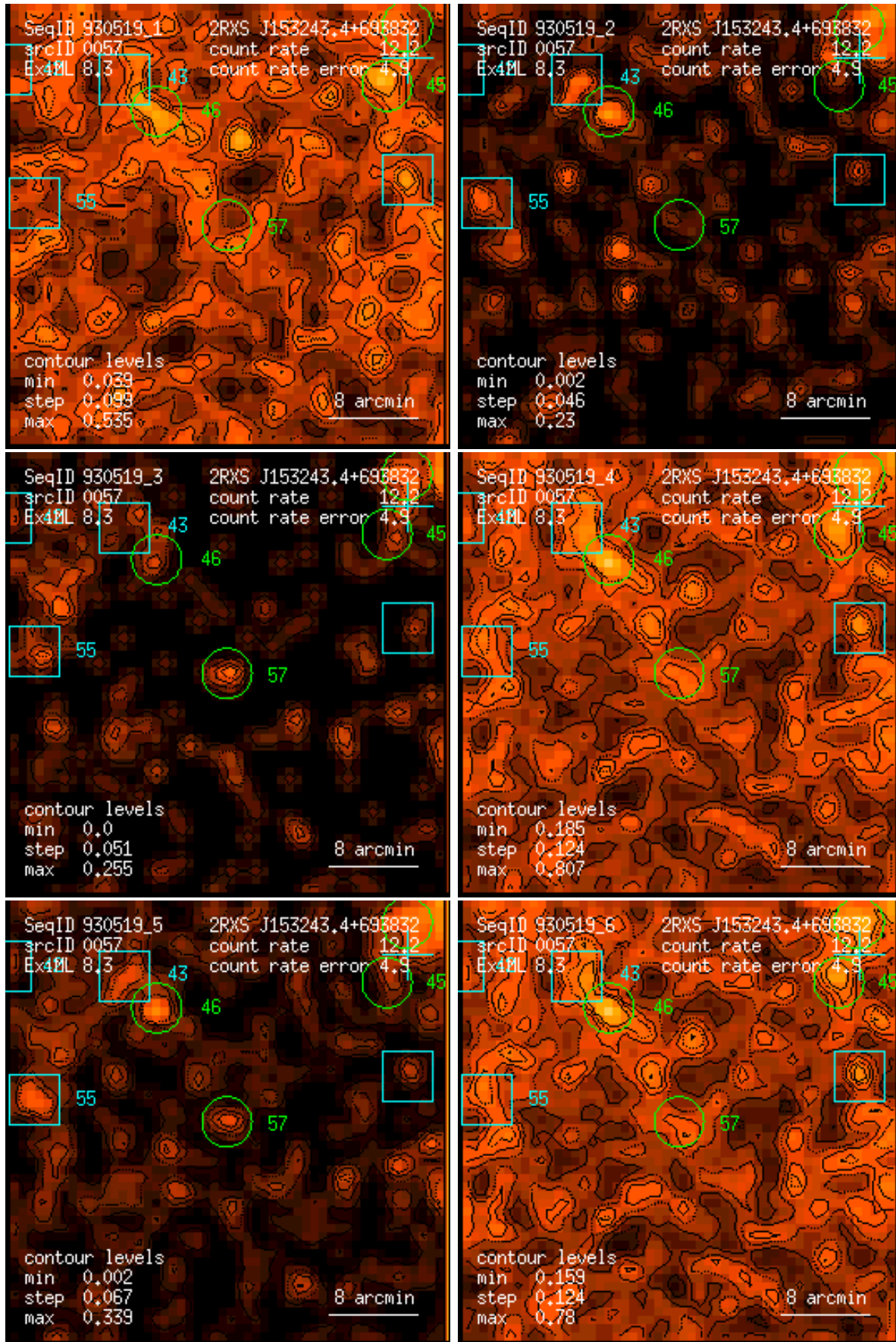
Figure 57: RASS 930519: detection 0057: band rate images, Gaussian filter: (1) PSPC channels 11 – 41, (2) 52 – 90, (3) 91 – 201, (4) 11 – 235, (5) 52 – 201, (6) 11 – 201. Broad band rates in counts/ks. Band rate contour levels in counts/ks/arcmin 2 .
