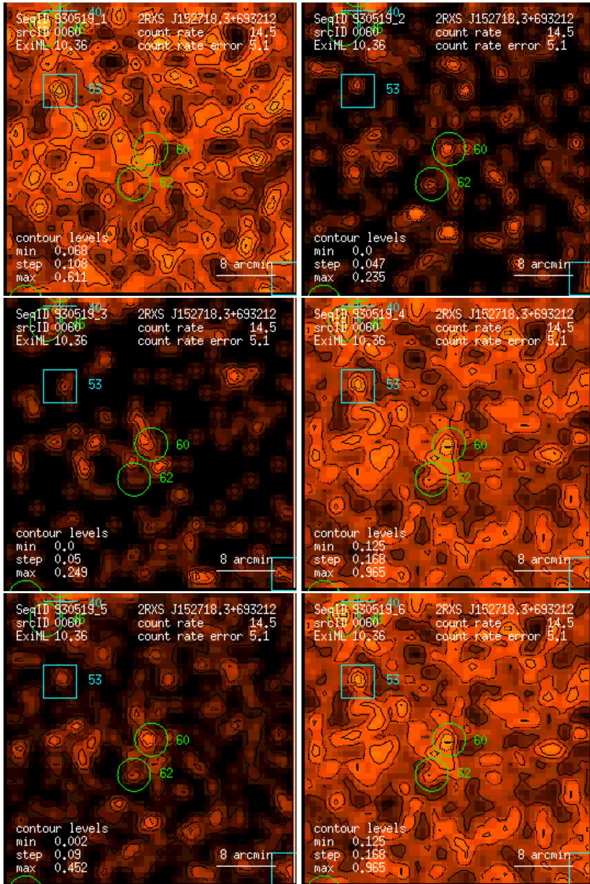
Figure 60: RASS 930519: detection 0060: band rate images, Gaussian filter: (1) PSPC channels 11 – 41, (2) 52 – 90, (3) 91 – 201, (4) 11 – 235, (5) 52 – 201, (6) 11 – 201. Broad band rates in counts/ks. Band rate contour levels in counts/ks/arcmin 2 .
