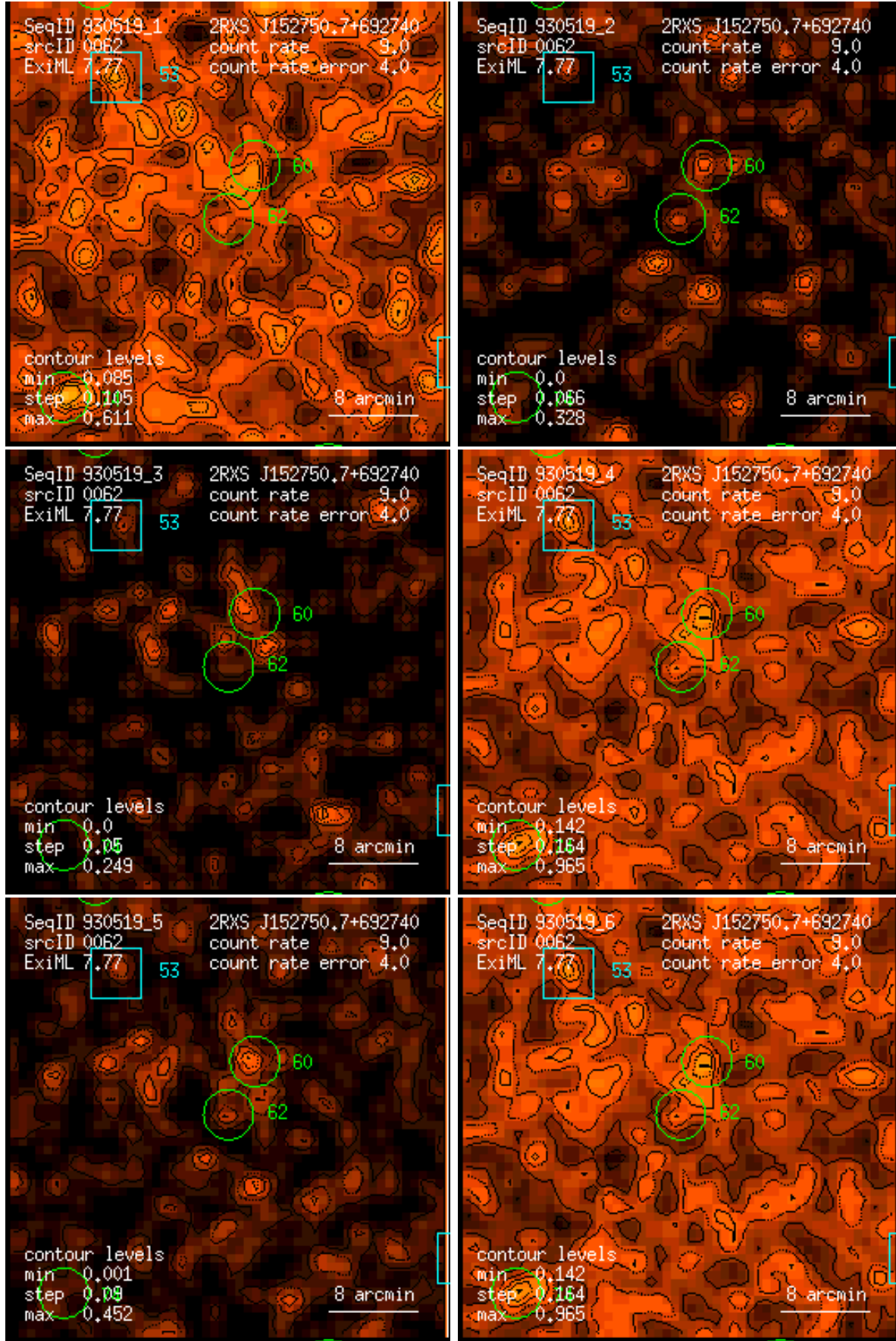
Figure 62: RASS 930519: detection 0062: band rate images, Gaussian filter: (1) PSPC channels 11 – 41, (2) 52 – 90, (3) 91 – 201, (4) 11 – 235, (5) 52 – 201, (6) 11 – 201. Broad band rates in counts/ks. Band rate contour levels in counts/ks/arcmin 2 .
