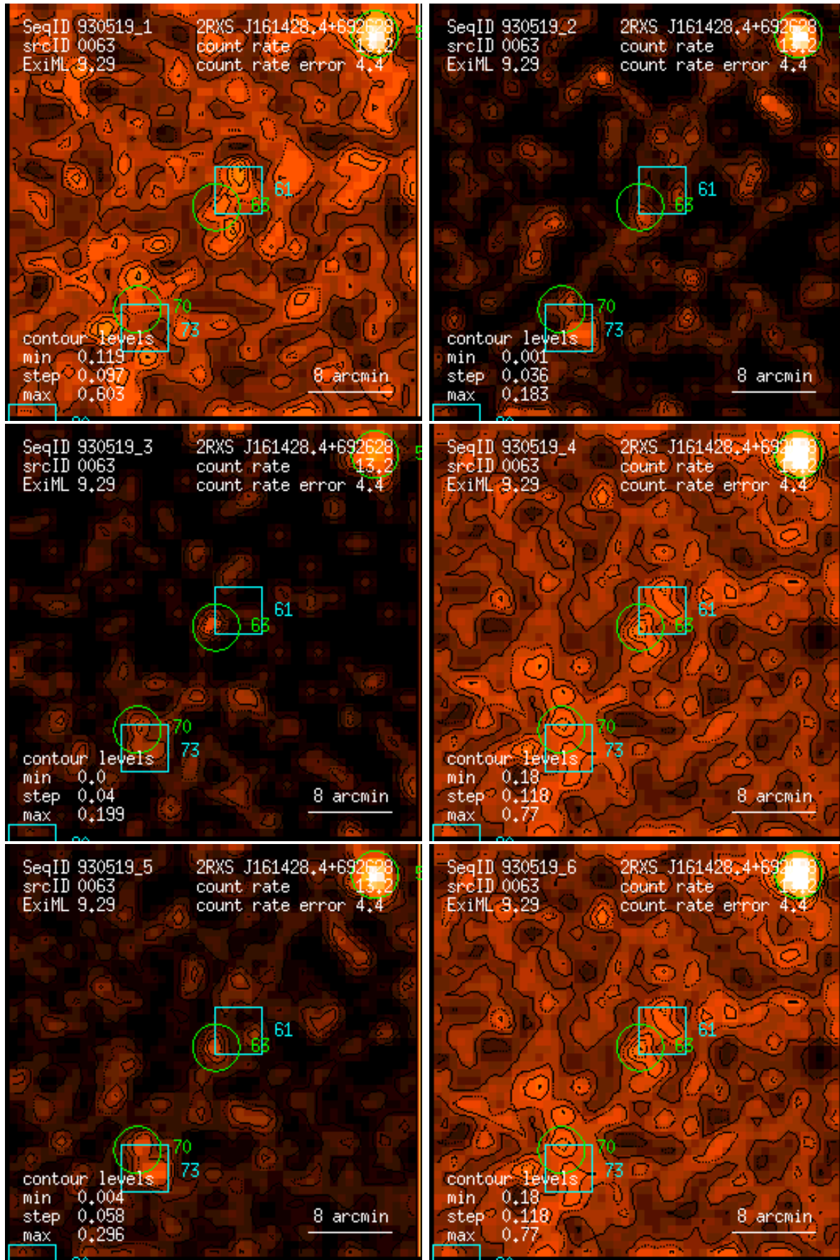
Figure 63: RASS 930519: detection 0063: band rate images, Gaussian filter: (1) PSPC channels 11 – 41, (2) 52 – 90, (3) 91 – 201, (4) 11 – 235, (5) 52 – 201, (6) 11 – 201. Broad band rates in counts/ks. Band rate contour levels in counts/ks/arcmin 2 .
