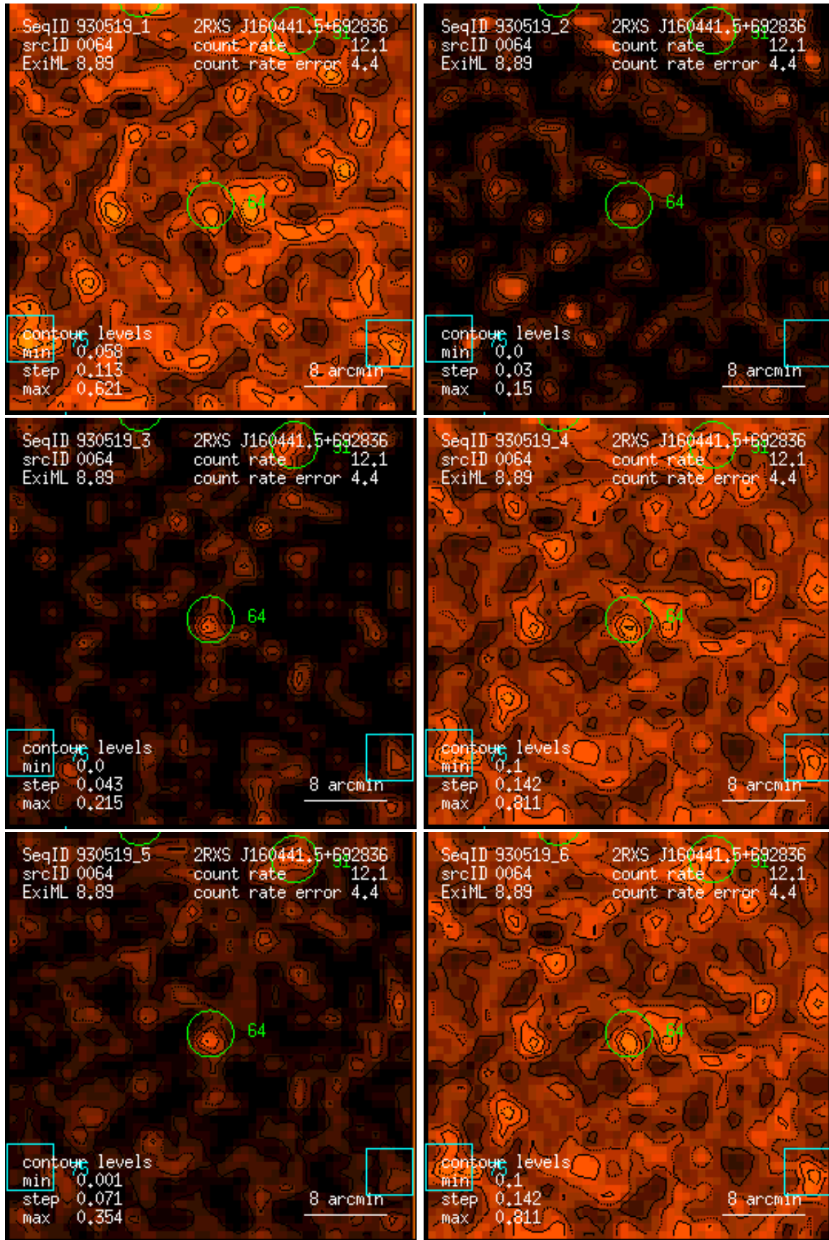
Figure 64: RASS 930519: detection 0064: band rate images, Gaussian filter: (1) PSPC channels 11 – 41, (2) 52 – 90, (3) 91 – 201, (4) 11 – 235, (5) 52 – 201, (6) 11 – 201. Broad band rates in counts/ks. Band rate contour levels in counts/ks/arcmin 2 .
