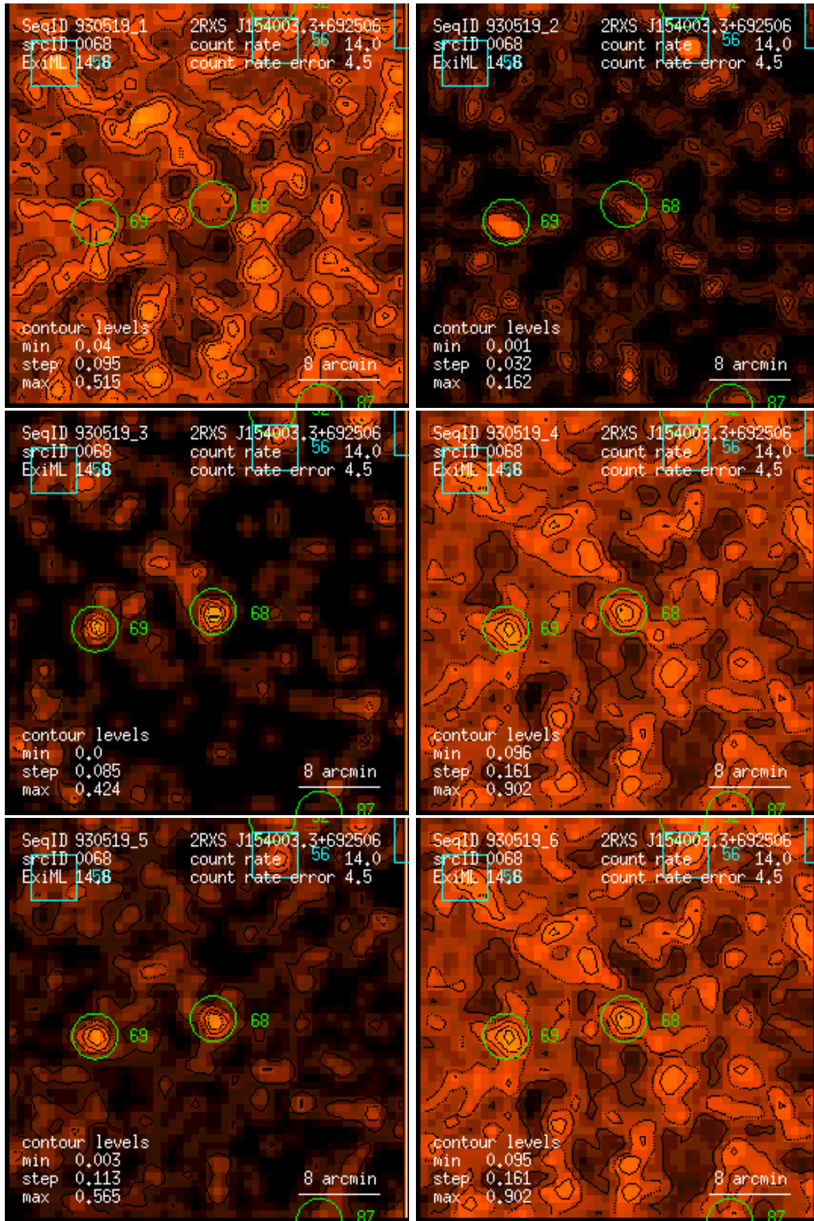
Figure 68: RASS 930519: detection 0068: band rate images, Gaussian filter: (1) PSPC channels 11 – 41, (2) 52 – 90, (3) 91 – 201, (4) 11 – 235, (5) 52 – 201, (6) 11 – 201. Broad band rates in counts/ks. Band rate contour levels in counts/ks/arcmin 2 .
