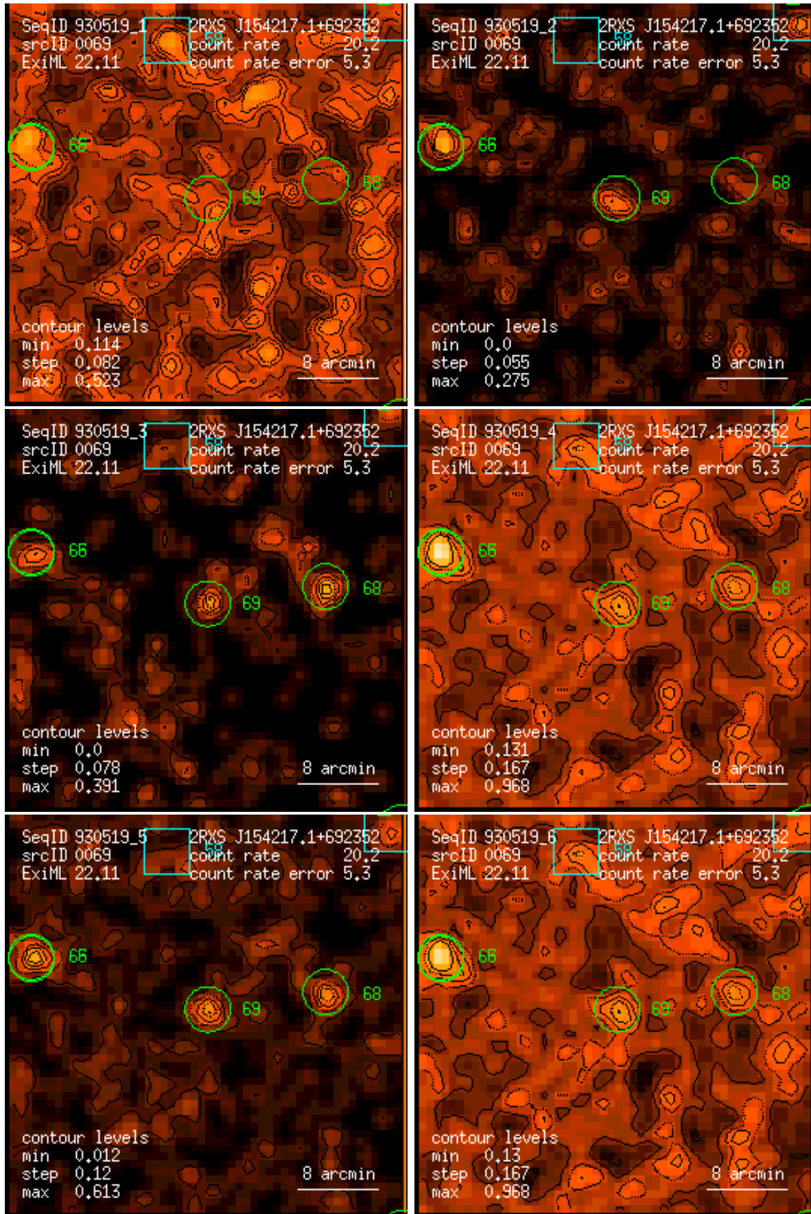
Figure 69: RASS 930519: detection 0069: band rate images, Gaussian filter: (1) PSPC channels 11 – 41, (2) 52 – 90, (3) 91 – 201, (4) 11 – 235, (5) 52 – 201, (6) 11 – 201. Broad band rates in counts/ks. Band rate contour levels in counts/ks/arcmin 2 .
