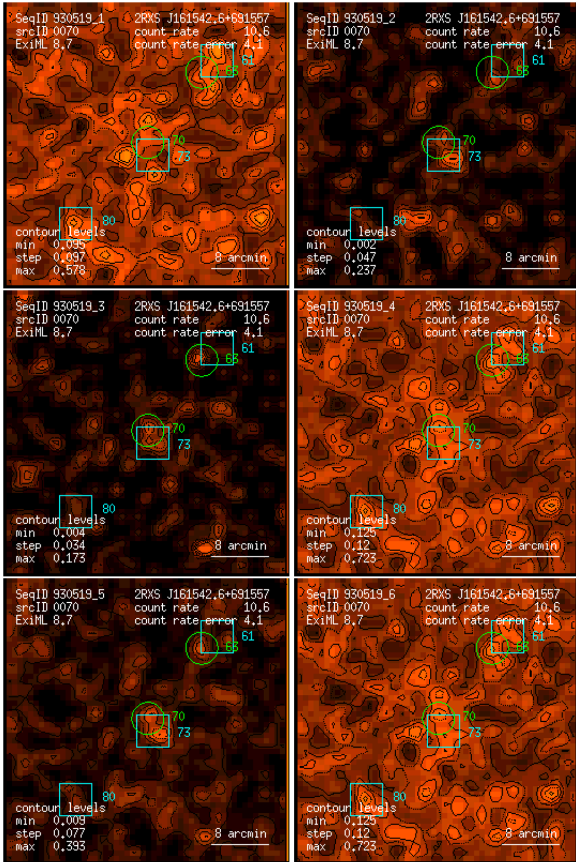
Figure 70: RASS 930519: detection 0070: band rate images, Gaussian filter: (1) PSPC channels 11 – 41, (2) 52 – 90, (3) 91 – 201, (4) 11 – 235, (5) 52 – 201, (6) 11 – 201. Broad band rates in counts/ks. Band rate contour levels in counts/ks/arcmin 2 .
