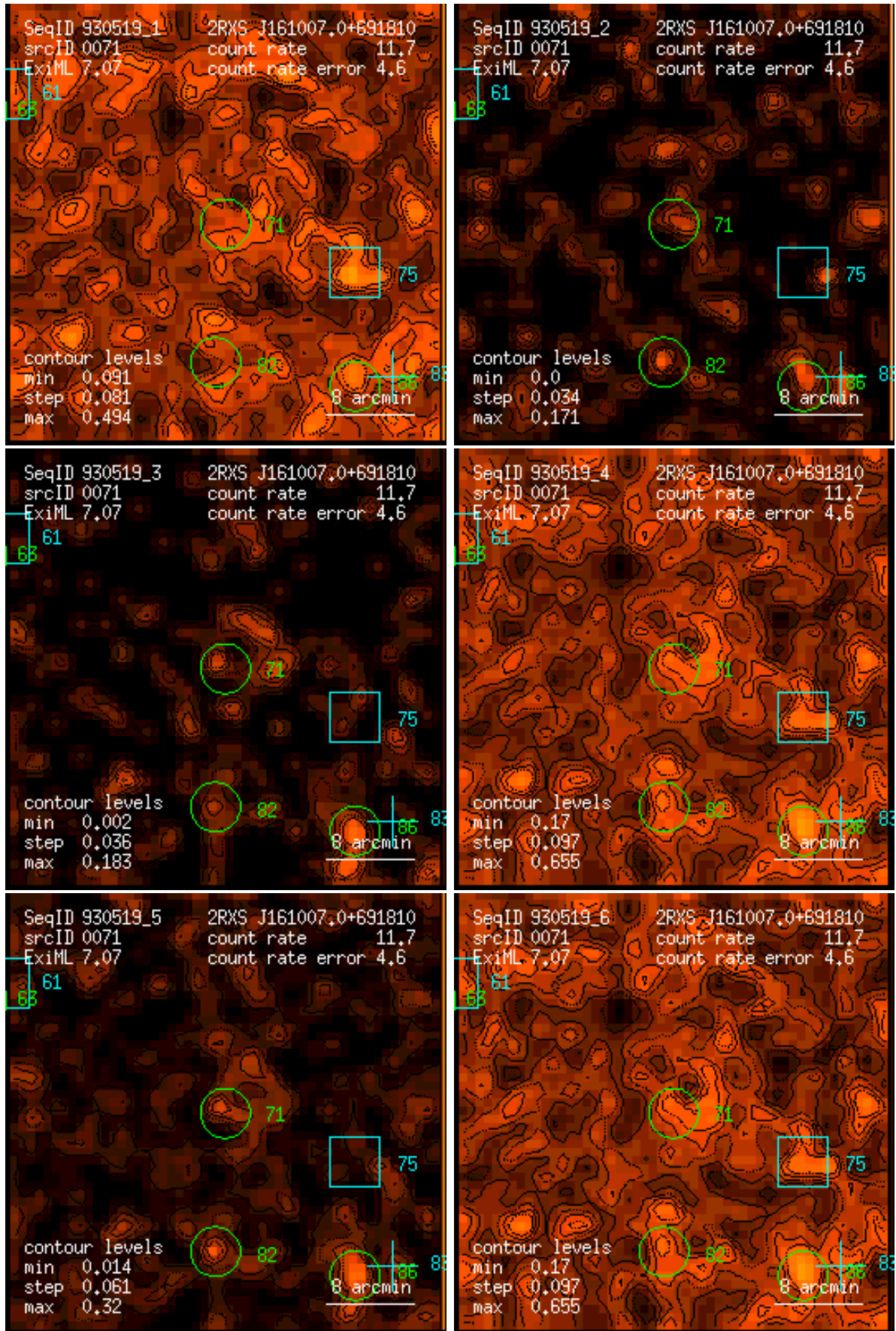
Figure 71: RASS 930519: detection 0071: band rate images, Gaussian filter: (1) PSPC channels 11 – 41, (2) 52 – 90, (3) 91 – 201, (4) 11 – 235, (5) 52 – 201, (6) 11 – 201. Broad band rates in counts/ks. Band rate contour levels in counts/ks/arcmin 2 .
