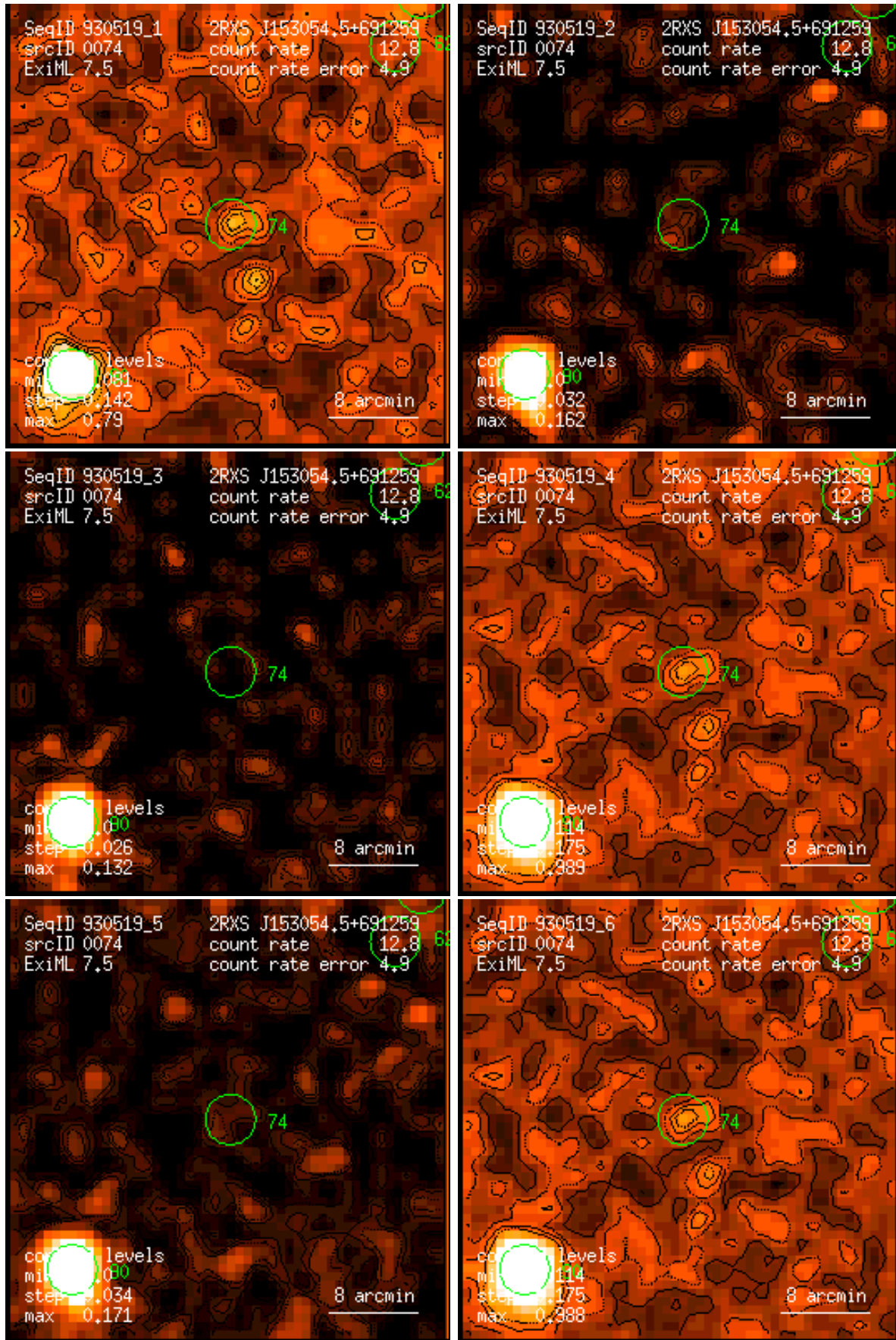
Figure 74: RASS 930519: detection 0074: band rate images, Gaussian filter: (1) PSPC channels 11 – 41, (2) 52 – 90, (3) 91 – 201, (4) 11 – 235, (5) 52 – 201, (6) 11 – 201. Broad band rates in counts/ks. Band rate contour levels in counts/ks/arcmin 2 .
