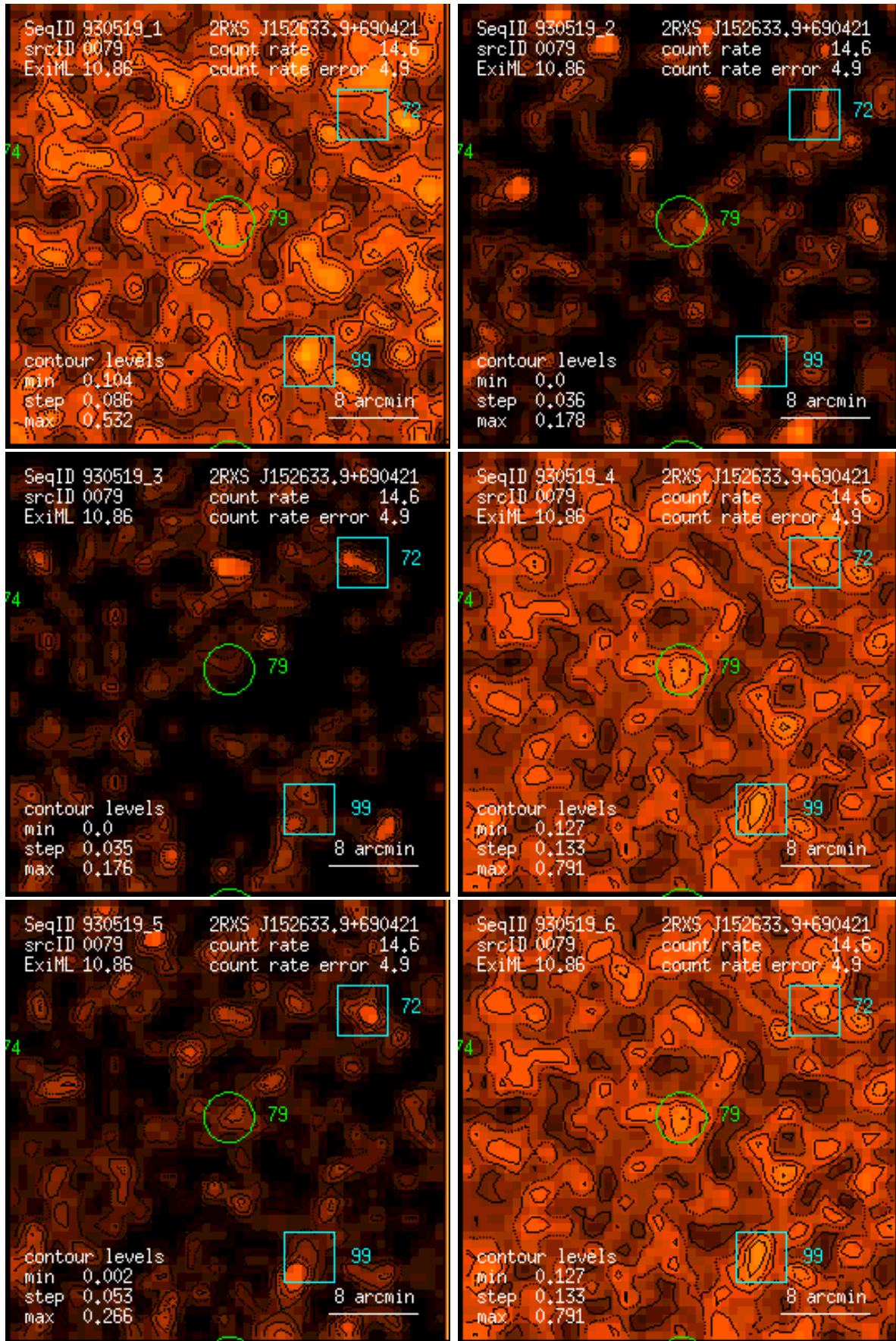
Figure 79: RASS 930519: detection 0079: band rate images, Gaussian filter: (1) PSPC channels 11 – 41, (2) 52 – 90, (3) 91 – 201, (4) 11 – 235, (5) 52 – 201, (6) 11 – 201. Broad band rates in counts/ks. Band rate contour levels in counts/ks/arcmin 2 .
