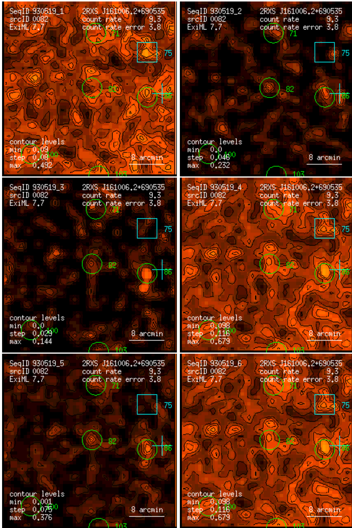
Figure 82: RASS 930519: detection 0082: band rate images, Gaussian filter: (1) PSPC channels 11 – 41, (2) 52 – 90, (3) 91 – 201, (4) 11 – 235, (5) 52 – 201, (6) 11 – 201. Broad band rates in counts/ks. Band rate contour levels in counts/ks/arcmin 2 .
