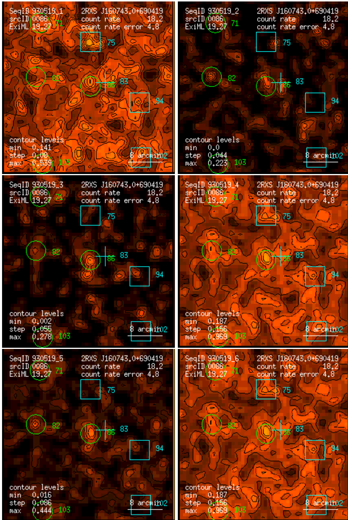
Figure 86: RASS 930519: detection 0086: band rate images, Gaussian filter: (1) PSPC channels 11 – 41, (2) 52 – 90, (3) 91 – 201, (4) 11 – 235, (5) 52 – 201, (6) 11 – 201. Broad band rates in counts/ks. Band rate contour levels in counts/ks/arcmin 2 .
