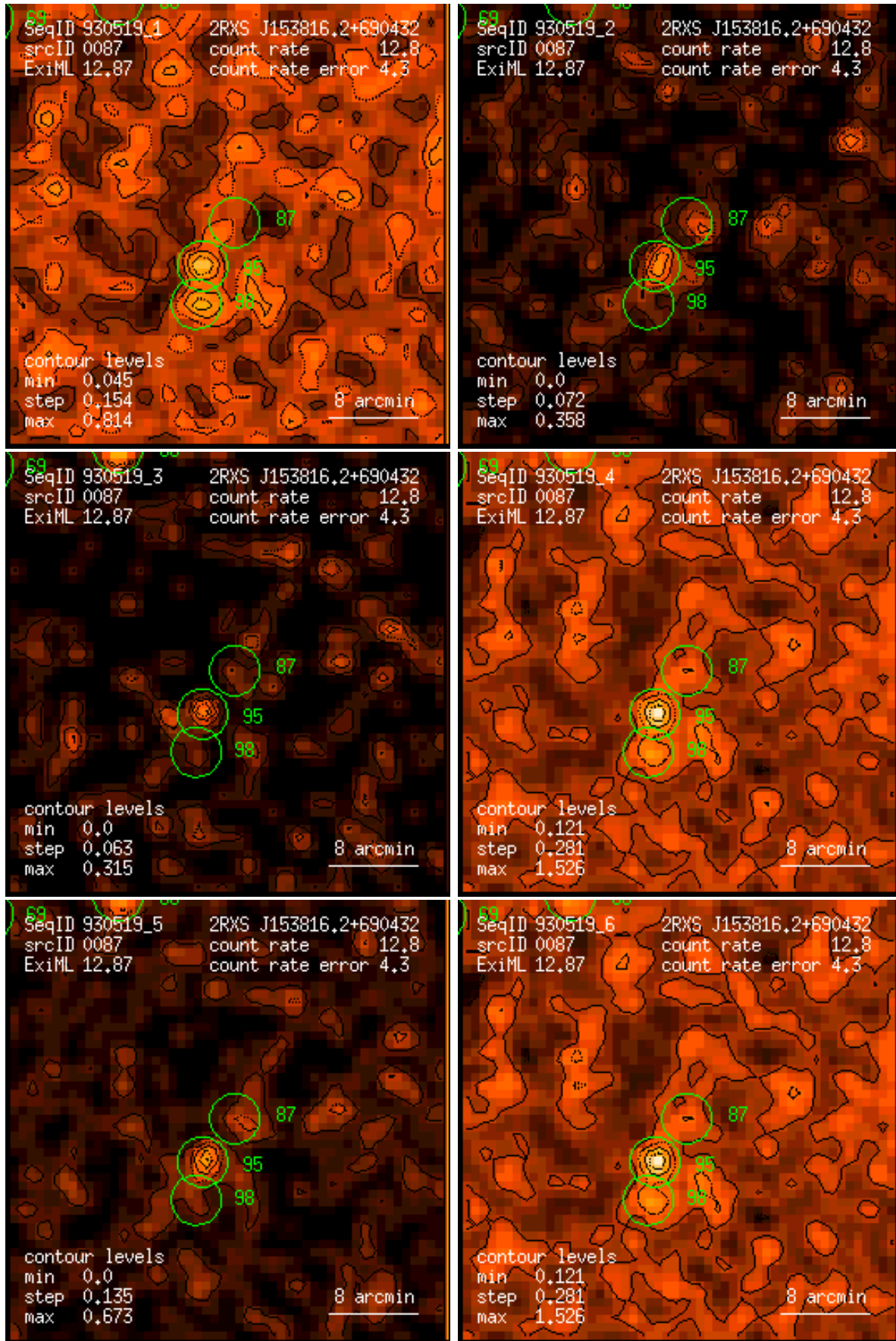
Figure 87: RASS 930519: detection 0087: band rate images, Gaussian filter: (1) PSPC channels 11 – 41, (2) 52 – 90, (3) 91 – 201, (4) 11 – 235, (5) 52 – 201, (6) 11 – 201. Broad band rates in counts/ks. Band rate contour levels in counts/ks/arcmin 2 .
