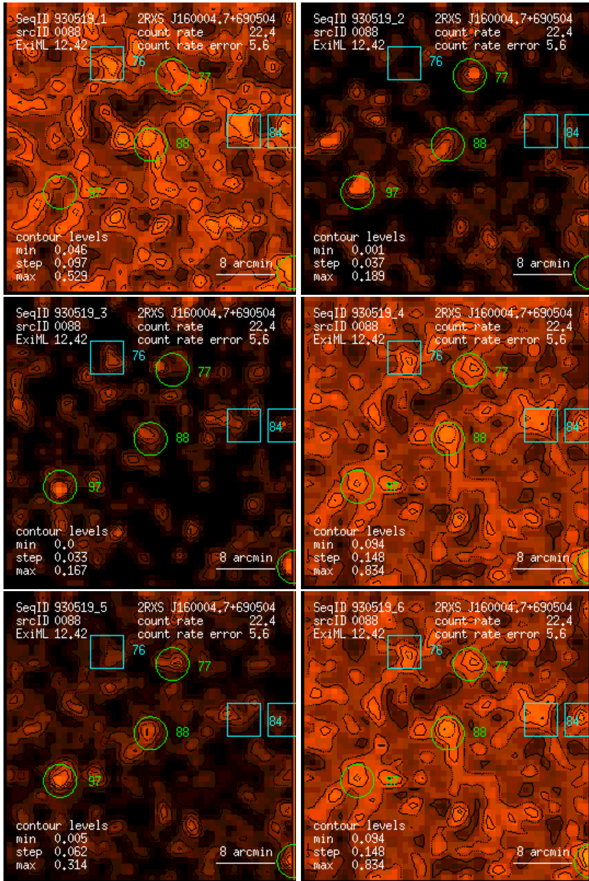
Figure 88: RASS 930519: detection 0088: band rate images, Gaussian filter: (1) PSPC channels 11 – 41, (2) 52 – 90, (3) 91 – 201, (4) 11 – 235, (5) 52 – 201, (6) 11 – 201. Broad band rates in counts/ks. Band rate contour levels in counts/ks/arcmin 2 .
