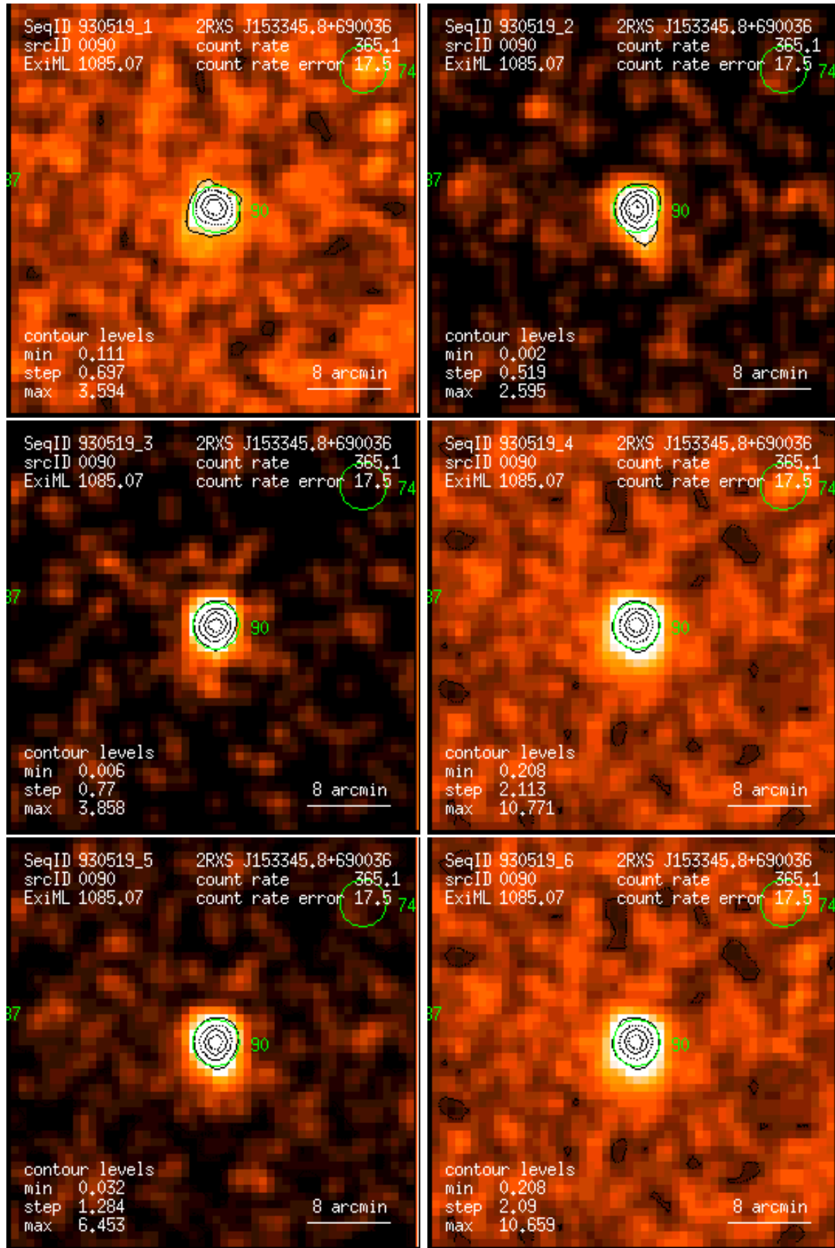
Figure 90: RASS 930519: detection 0090: band rate images, Gaussian filter: (1) PSPC channels 11 – 41, (2) 52 – 90, (3) 91 – 201, (4) 11 – 235, (5) 52 – 201, (6) 11 – 201. Broad band rates in counts/ks. Band rate contour levels in counts/ks/arcmin 2 .
