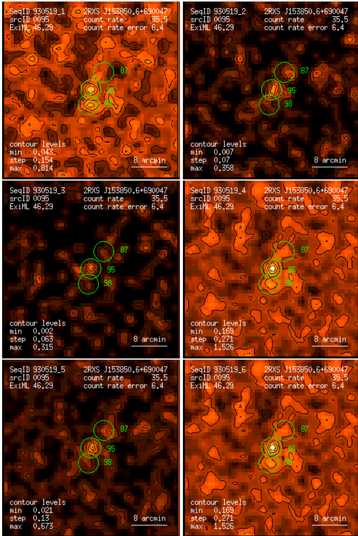
Figure 95: RASS 930519: detection 0095: band rate images, Gaussian filter: (1) PSPC channels 11 – 41, (2) 52 – 90, (3) 91 – 201, (4) 11 – 235, (5) 52 – 201, (6) 11 – 201. Broad band rates in counts/ks. Band rate contour levels in counts/ks/arcmin 2 .
