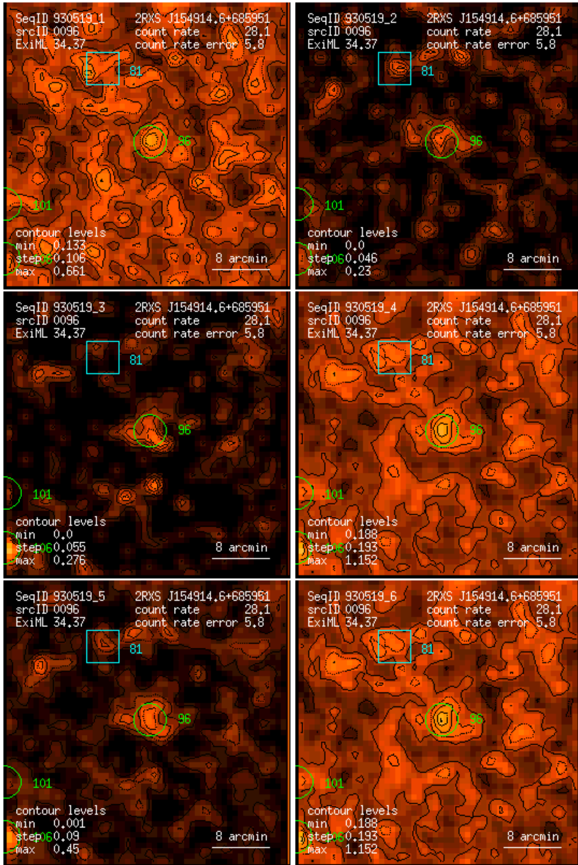
Figure 96: RASS 930519: detection 0096: band rate images, Gaussian filter: (1) PSPC channels 11 – 41, (2) 52 – 90, (3) 91 – 201, (4) 11 – 235, (5) 52 – 201, (6) 11 – 201. Broad band rates in counts/ks. Band rate contour levels in counts/ks/arcmin 2 .
