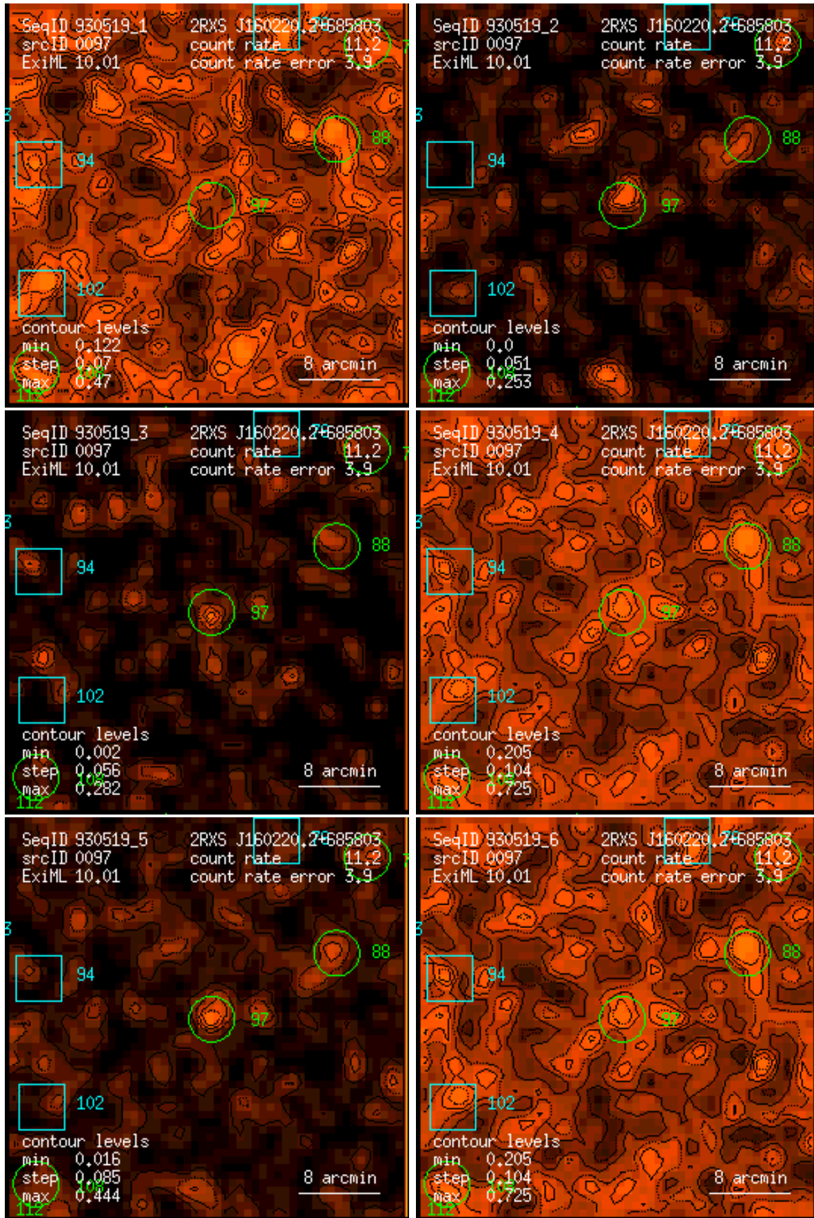
Figure 97: RASS 930519: detection 0097: band rate images, Gaussian filter: (1) PSPC channels 11 – 41, (2) 52 – 90, (3) 91 – 201, (4) 11 – 235, (5) 52 – 201, (6) 11 – 201. Broad band rates in counts/ks. Band rate contour levels in counts/ks/arcmin 2 .
