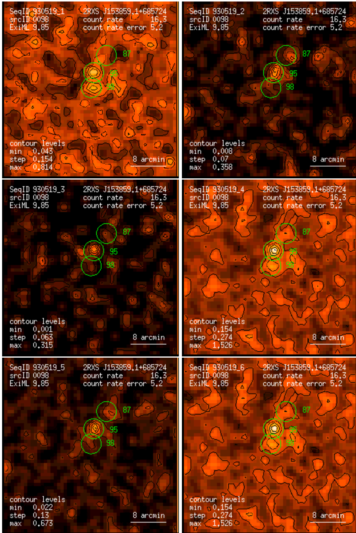
Figure 98: RASS 930519: detection 0098: band rate images, Gaussian filter: (1) PSPC channels 11 – 41, (2) 52 – 90, (3) 91 – 201, (4) 11 – 235, (5) 52 – 201, (6) 11 – 201. Broad band rates in counts/ks. Band rate contour levels in counts/ks/arcmin 2 .
