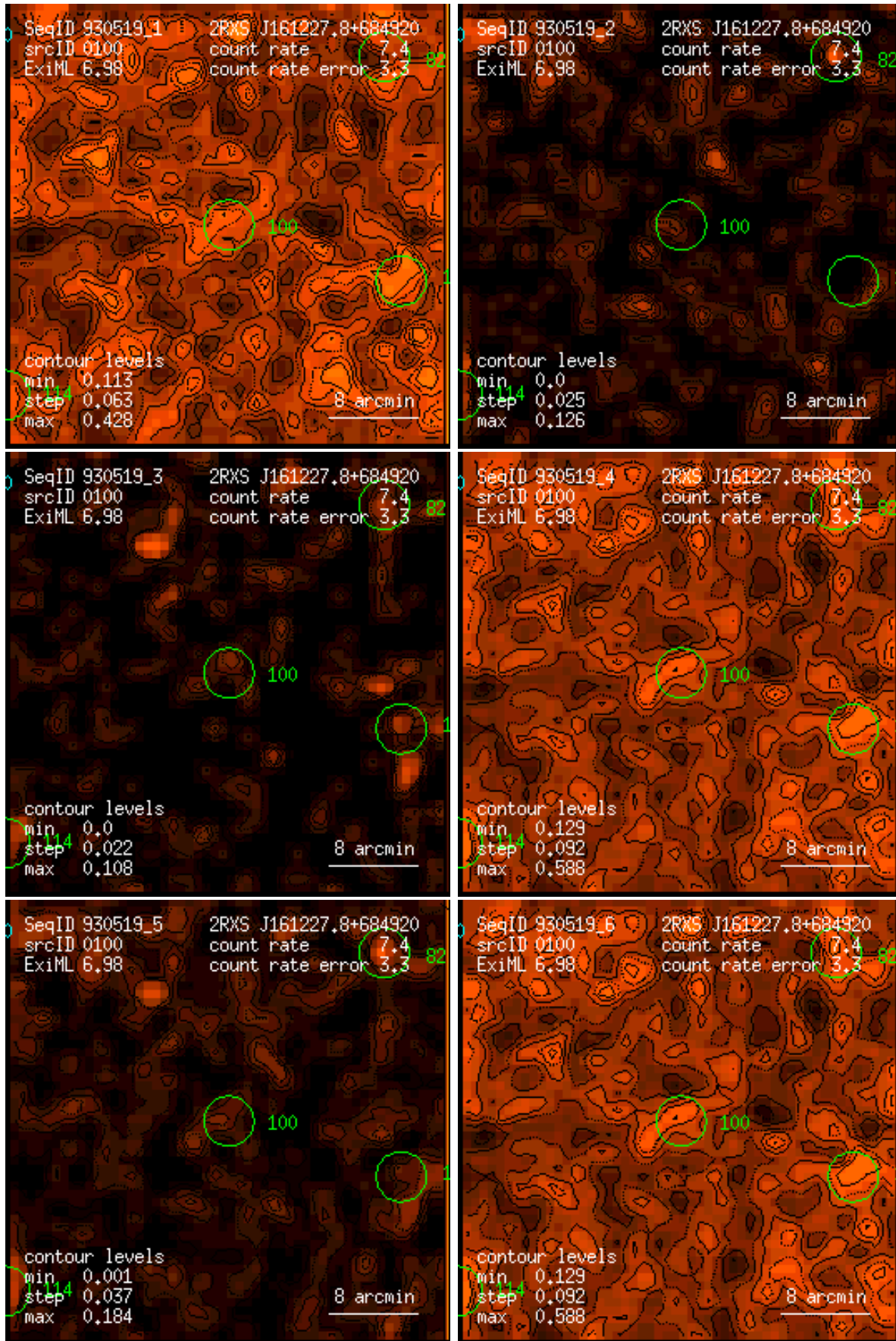
Figure 100: RASS 930519: detection 0100: band rate images, Gaussian filter: (1) PSPC channels 11 – 41, (2) 52 – 90, (3) 91 – 201, (4) 11 – 235, (5) 52 – 201, (6) 11 – 201. Broad band rates in counts/ks. Band rate contour levels in counts/ks/arcmin 2 .
