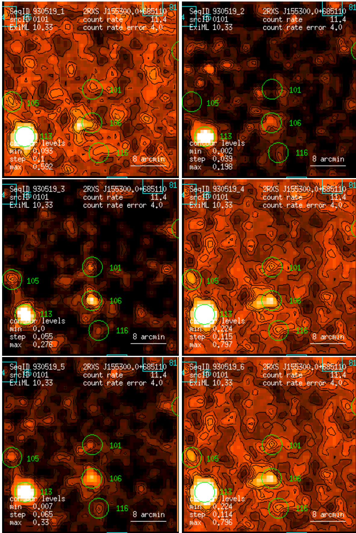
Figure 101: RASS 930519: detection 0101: band rate images, Gaussian filter: (1) PSPC channels 11 – 41, (2) 52 – 90, (3) 91 – 201, (4) 11 – 235, (5) 52 – 201, (6) 11 – 201. Broad band rates in counts/ks. Band rate contour levels in counts/ks/arcmin 2 .
