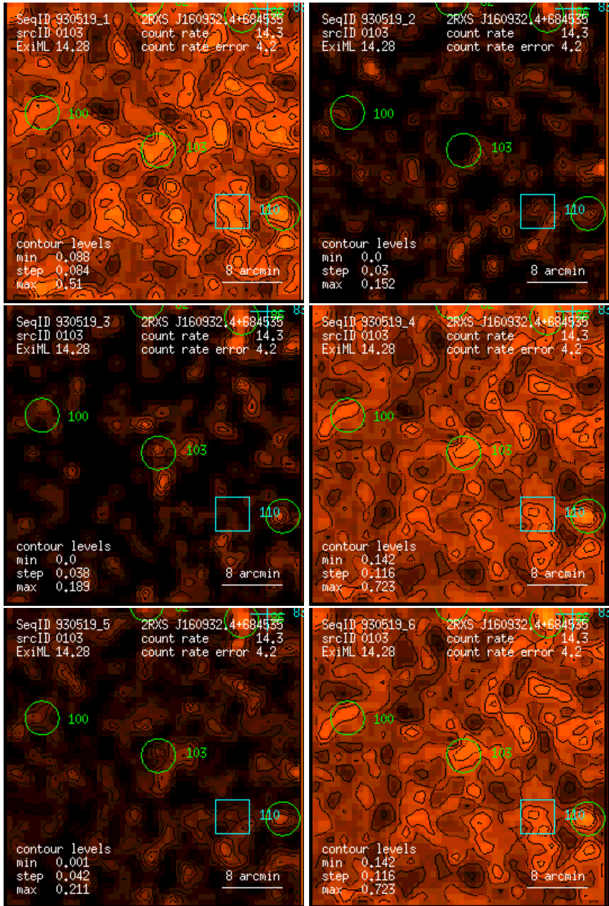
Figure 103: RASS 930519: detection 0103: band rate images, Gaussian filter: (1) PSPC channels 11 – 41, (2) 52 – 90, (3) 91 – 201, (4) 11 – 235, (5) 52 – 201, (6) 11 – 201. Broad band rates in counts/ks. Band rate contour levels in counts/ks/arcmin 2 .
