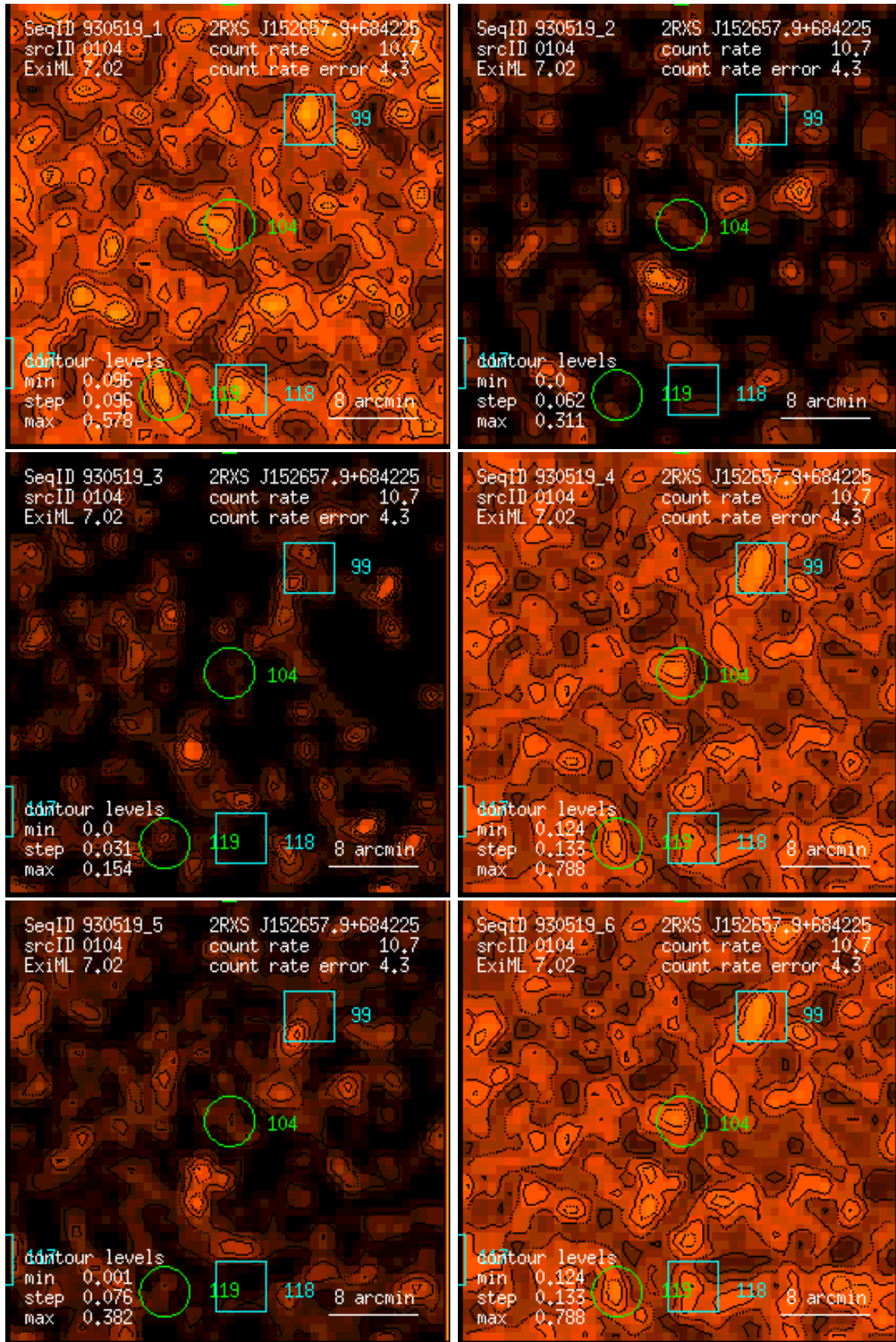
Figure 104: RASS 930519: detection 0104: band rate images, Gaussian filter: (1) PSPC channels 11 – 41, (2) 52 – 90, (3) 91 – 201, (4) 11 – 235, (5) 52 – 201, (6) 11 – 201. Broad band rates in counts/ks. Band rate contour levels in counts/ks/arcmin 2 .
