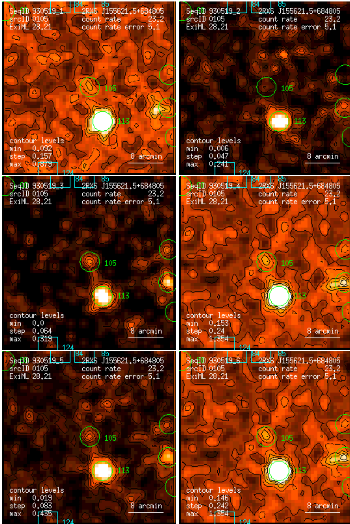
Figure 105: RASS 930519: detection 0105: band rate images, Gaussian filter: (1) PSPC channels 11 – 41, (2) 52 – 90, (3) 91 – 201, (4) 11 – 235, (5) 52 – 201, (6) 11 – 201. Broad band rates in counts/ks. Band rate contour levels in counts/ks/arcmin 2 .
