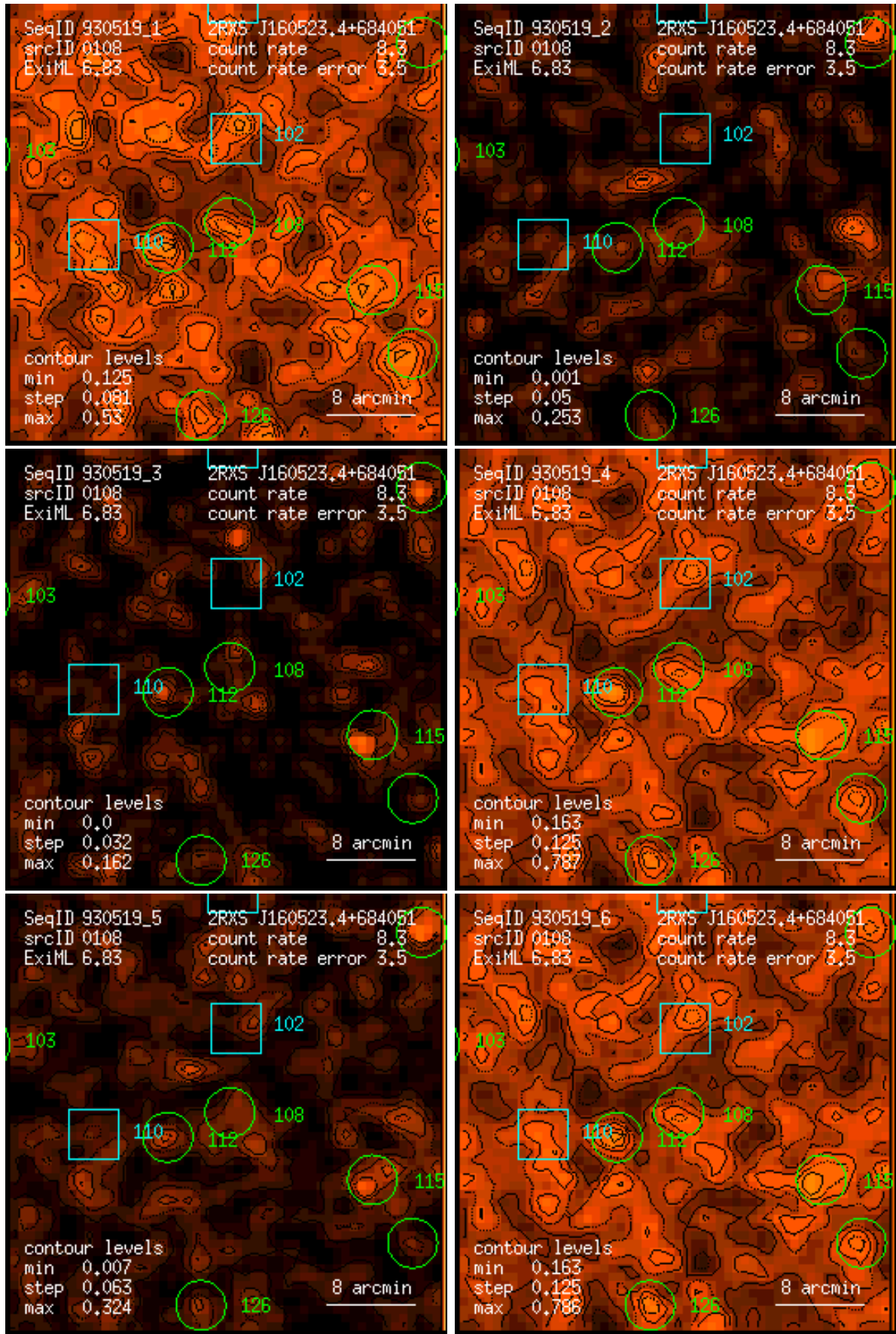
Figure 108: RASS 930519: detection 0108: band rate images, Gaussian filter: (1) PSPC channels 11 – 41, (2) 52 – 90, (3) 91 – 201, (4) 11 – 235, (5) 52 – 201, (6) 11 – 201. Broad band rates in counts/ks. Band rate contour levels in counts/ks/arcmin 2 .
