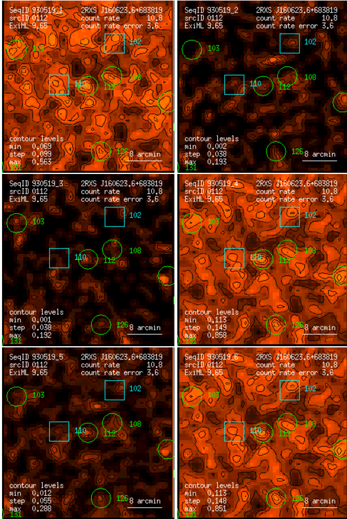
Figure 112: RASS 930519: detection 0112: band rate images, Gaussian filter: (1) PSPC channels 11 – 41, (2) 52 – 90, (3) 91 – 201, (4) 11 – 235, (5) 52 – 201, (6) 11 – 201. Broad band rates in counts/ks. Band rate contour levels in counts/ks/arcmin 2 .
