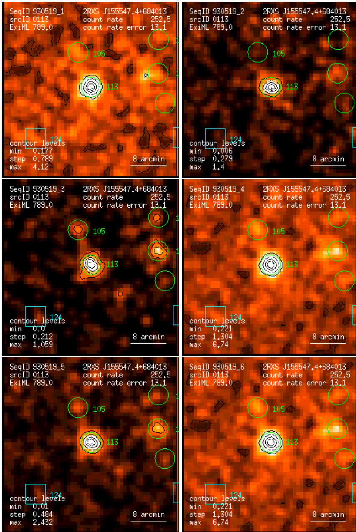
Figure 113: RASS 930519: detection 0113: band rate images, Gaussian filter: (1) PSPC channels 11 – 41, (2) 52 – 90, (3) 91 – 201, (4) 11 – 235, (5) 52 – 201, (6) 11 – 201. Broad band rates in counts/ks. Band rate contour levels in counts/ks/arcmin 2 .
