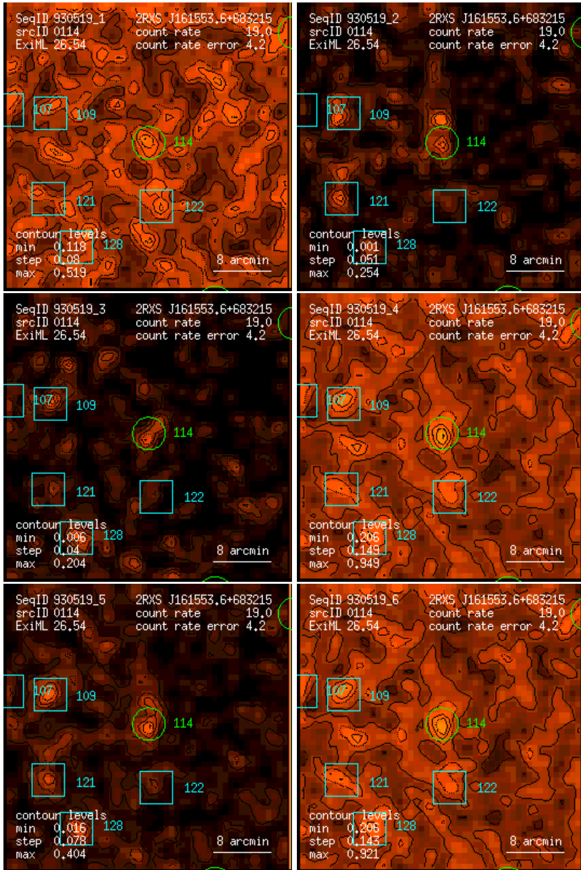
Figure 114: RASS 930519: detection 0114: band rate images, Gaussian filter: (1) PSPC channels 11 – 41, (2) 52 – 90, (3) 91 – 201, (4) 11 – 235, (5) 52 – 201, (6) 11 – 201. Broad band rates in counts/ks. Band rate contour levels in counts/ks/arcmin 2 .
