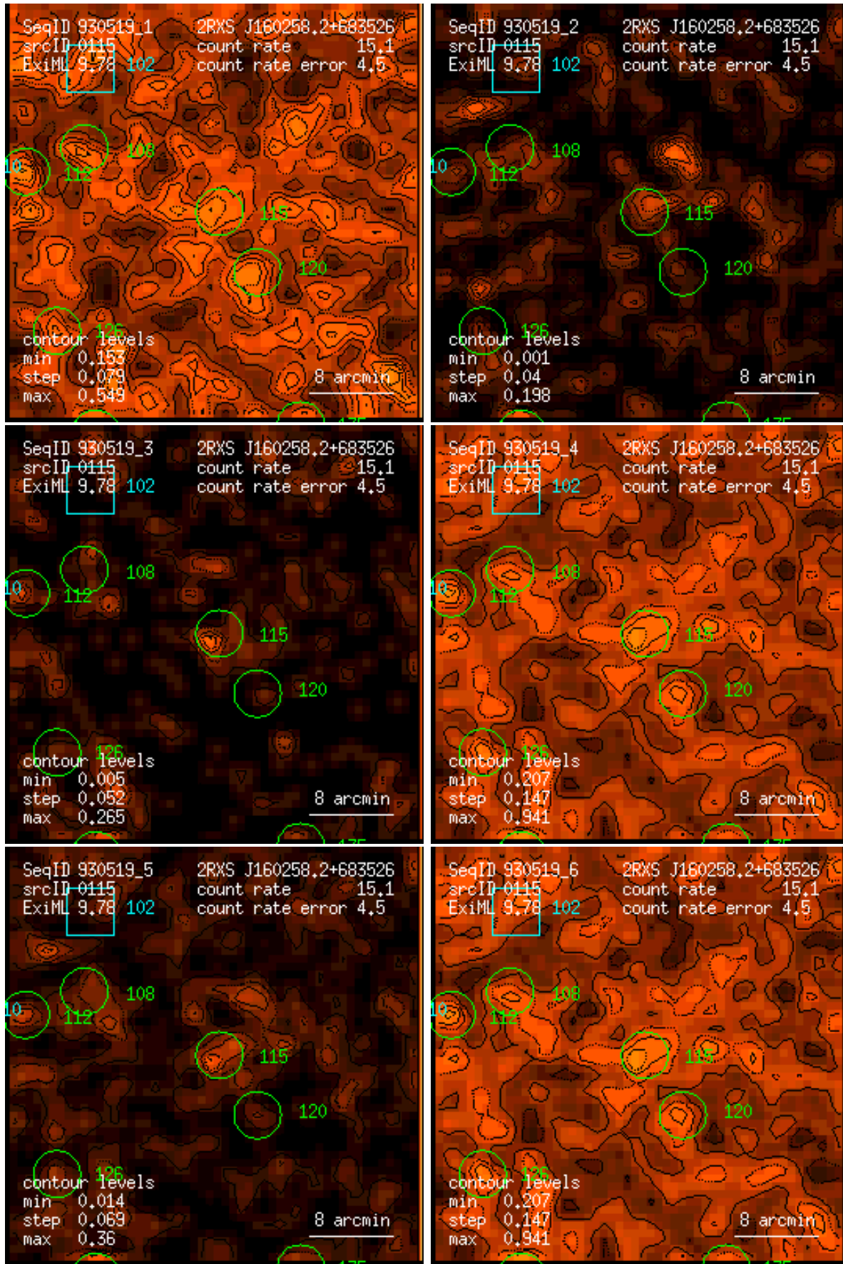
Figure 115: RASS 930519: detection 0115: band rate images, Gaussian filter: (1) PSPC channels 11 – 41, (2) 52 – 90, (3) 91 – 201, (4) 11 – 235, (5) 52 – 201, (6) 11 – 201. Broad band rates in counts/ks. Band rate contour levels in counts/ks/arcmin 2 .
