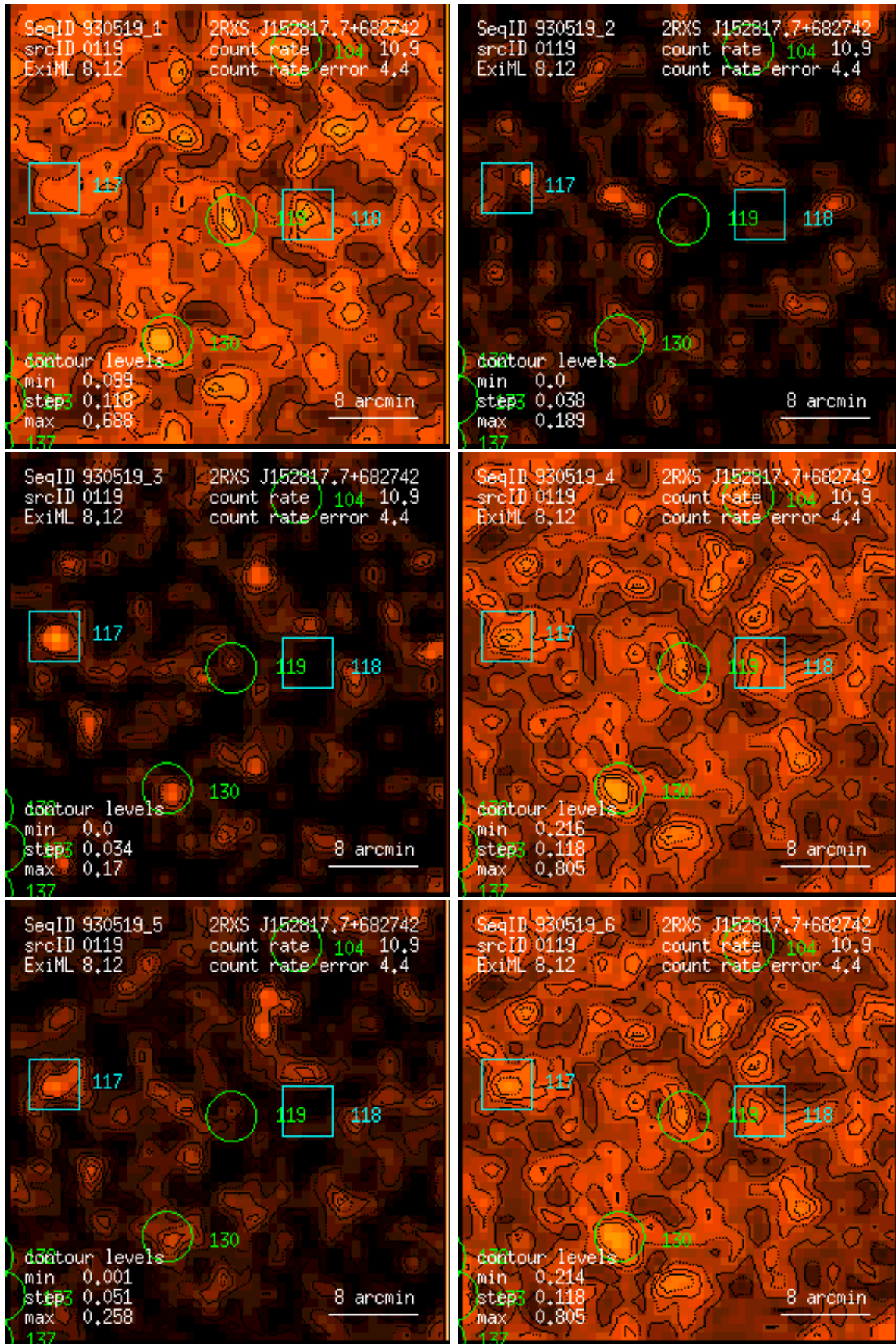
Figure 119: RASS 930519: detection 0119: band rate images, Gaussian filter: (1) PSPC channels 11 – 41, (2) 52 – 90, (3) 91 – 201, (4) 11 – 235, (5) 52 – 201, (6) 11 – 201. Broad band rates in counts/ks. Band rate contour levels in counts/ks/arcmin 2 .
