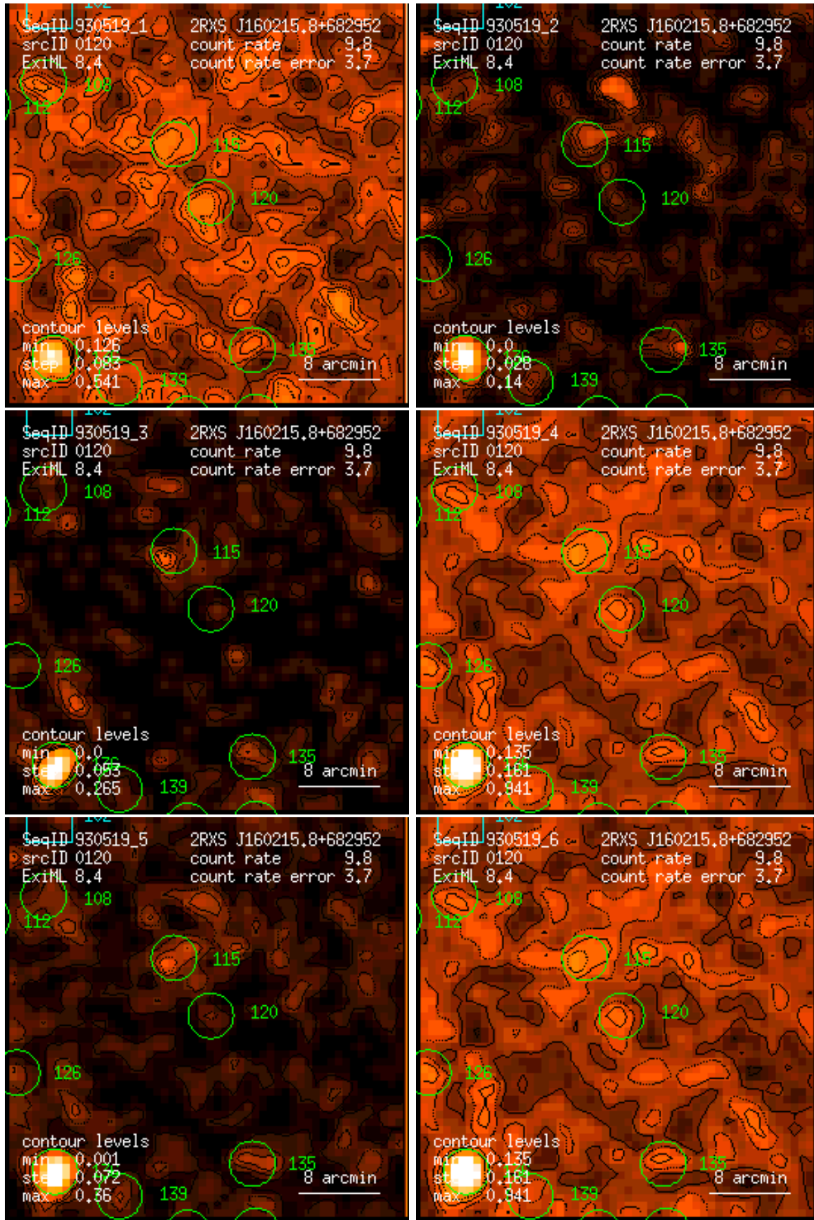
Figure 120: RASS 930519: detection 0120: band rate images, Gaussian filter: (1) PSPC channels 11 – 41, (2) 52 – 90, (3) 91 – 201, (4) 11 – 235, (5) 52 – 201, (6) 11 – 201. Broad band rates in counts/ks. Band rate contour levels in counts/ks/arcmin 2 .
