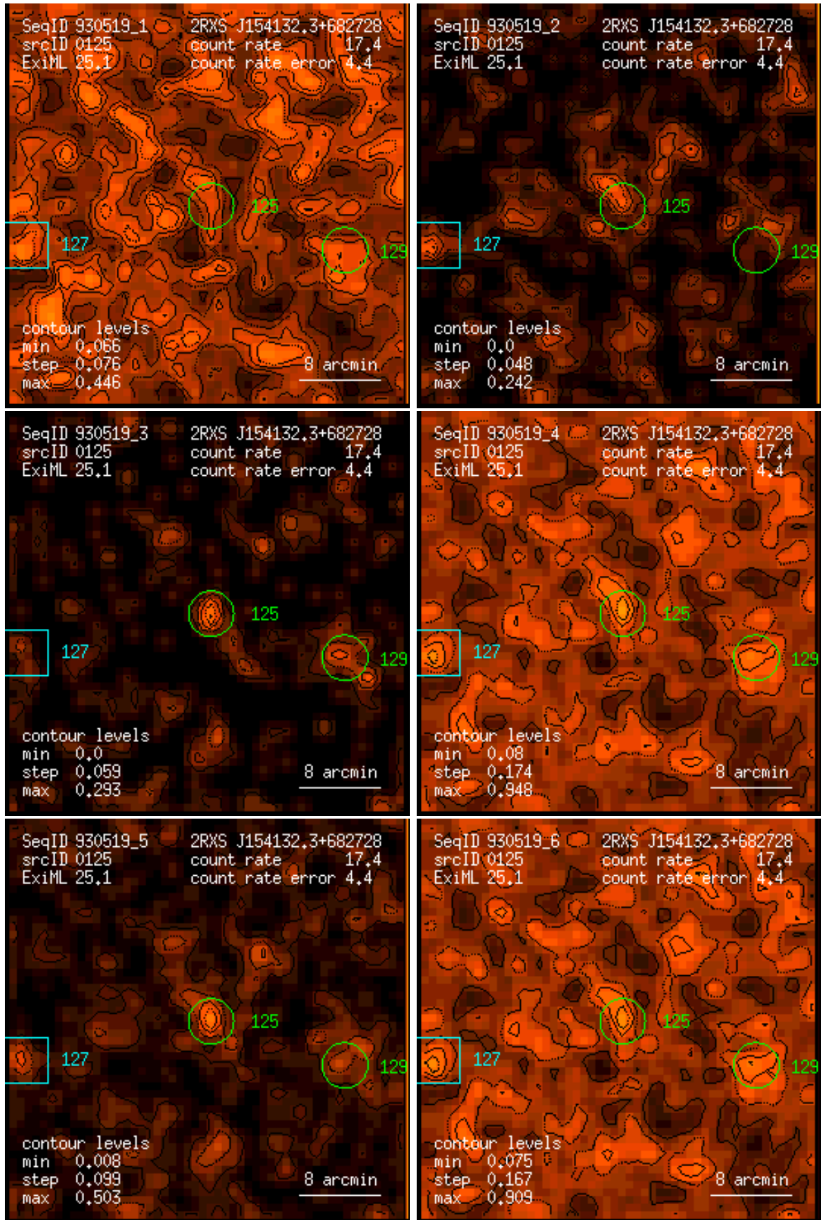
Figure 125: RASS 930519: detection 0125: band rate images, Gaussian filter: (1) PSPC channels 11 – 41, (2) 52 – 90, (3) 91 – 201, (4) 11 – 235, (5) 52 – 201, (6) 11 – 201. Broad band rates in counts/ks. Band rate contour levels in counts/ks/arcmin 2 .
