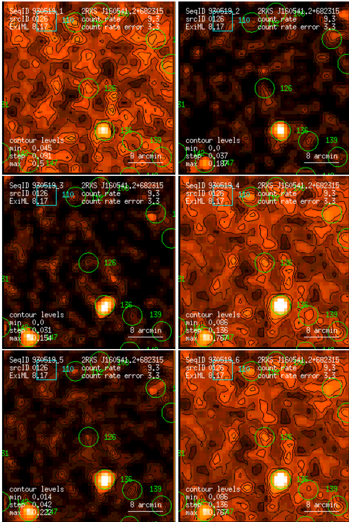
Figure 126: RASS 930519: detection 0126: band rate images, Gaussian filter: (1) PSPC channels 11 – 41, (2) 52 – 90, (3) 91 – 201, (4) 11 – 235, (5) 52 – 201, (6) 11 – 201. Broad band rates in counts/ks. Band rate contour levels in counts/ks/arcmin 2 .
