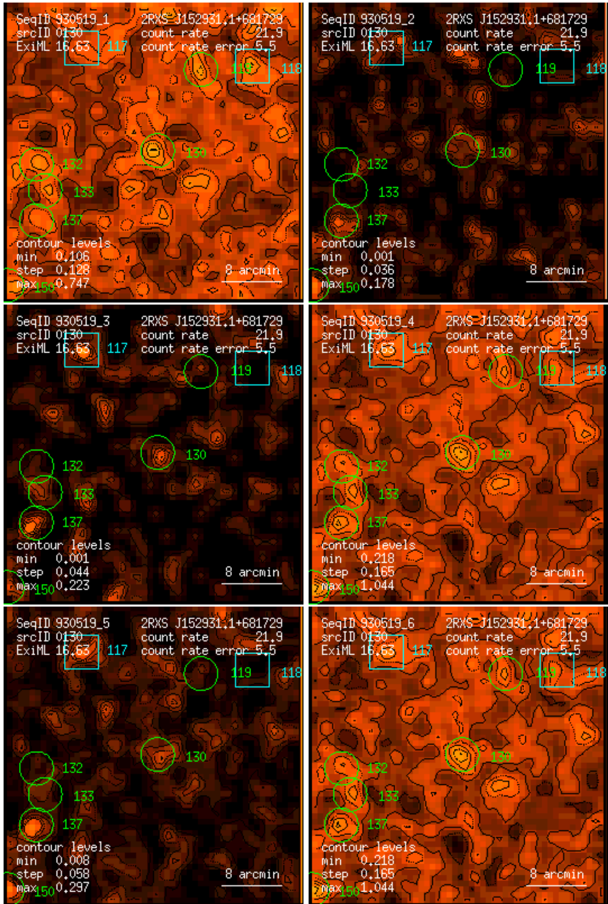
Figure 130: RASS 930519: detection 0130: band rate images, Gaussian filter: (1) PSPC channels 11 – 41, (2) 52 – 90, (3) 91 – 201, (4) 11 – 235, (5) 52 – 201, (6) 11 – 201. Broad band rates in counts/ks. Band rate contour levels in counts/ks/arcmin 2 .
