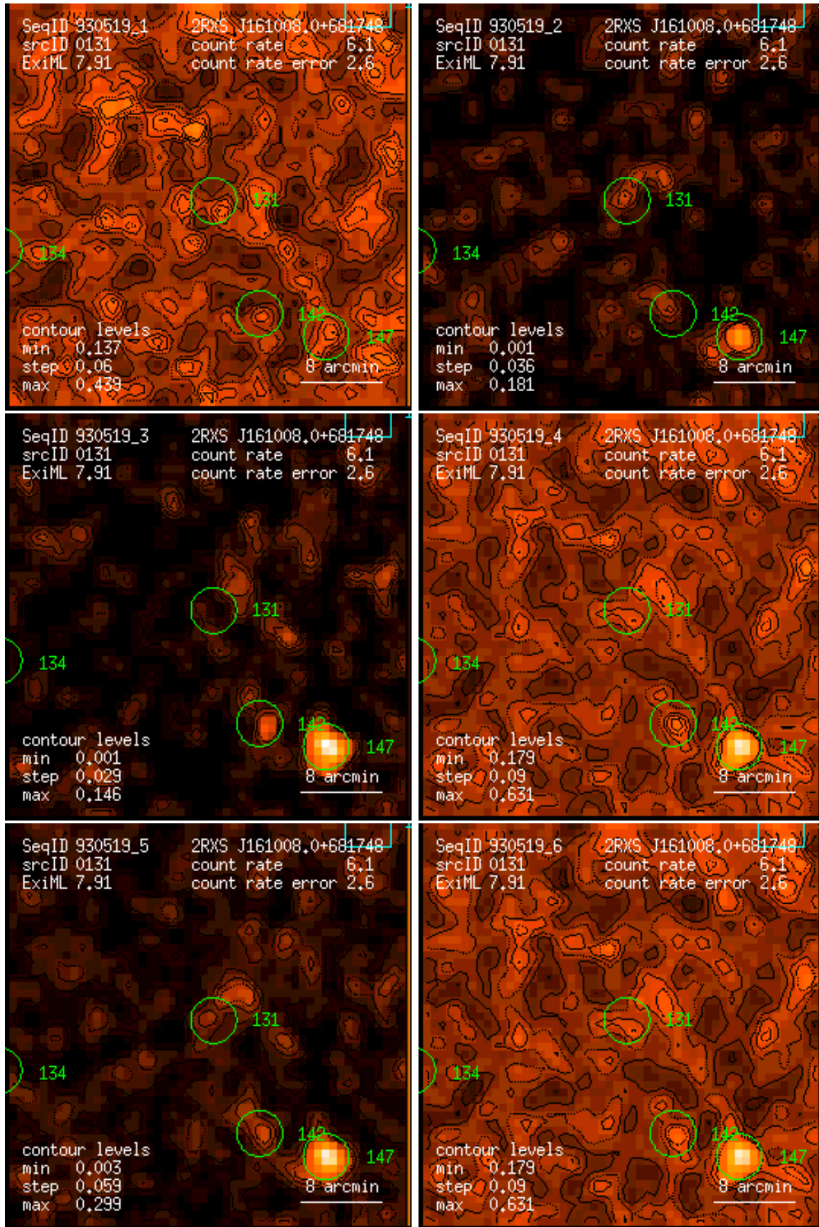
Figure 131: RASS 930519: detection 0131: band rate images, Gaussian filter: (1) PSPC channels 11 – 41, (2) 52 – 90, (3) 91 – 201, (4) 11 – 235, (5) 52 – 201, (6) 11 – 201. Broad band rates in counts/ks. Band rate contour levels in counts/ks/arcmin 2 .
