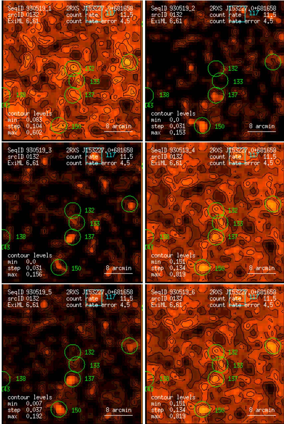
Figure 132: RASS 930519: detection 0132: band rate images, Gaussian filter: (1) PSPC channels 11 – 41, (2) 52 – 90, (3) 91 – 201, (4) 11 – 235, (5) 52 – 201, (6) 11 – 201. Broad band rates in counts/ks. Band rate contour levels in counts/ks/arcmin 2 .
