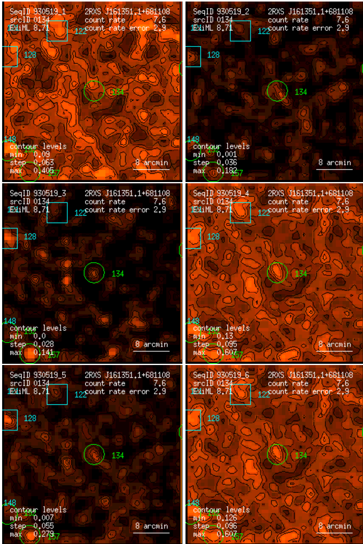
Figure 134: RASS 930519: detection 0134: band rate images, Gaussian filter: (1) PSPC channels 11 – 41, (2) 52 – 90, (3) 91 – 201, (4) 11 – 235, (5) 52 – 201, (6) 11 – 201. Broad band rates in counts/ks. Band rate contour levels in counts/ks/arcmin 2 .
