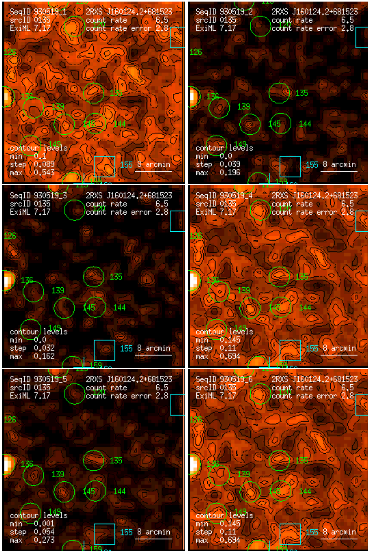
Figure 135: RASS 930519: detection 0135: band rate images, Gaussian filter: (1) PSPC channels 11 – 41, (2) 52 – 90, (3) 91 – 201, (4) 11 – 235, (5) 52 – 201, (6) 11 – 201. Broad band rates in counts/ks. Band rate contour levels in counts/ks/arcmin 2 .
