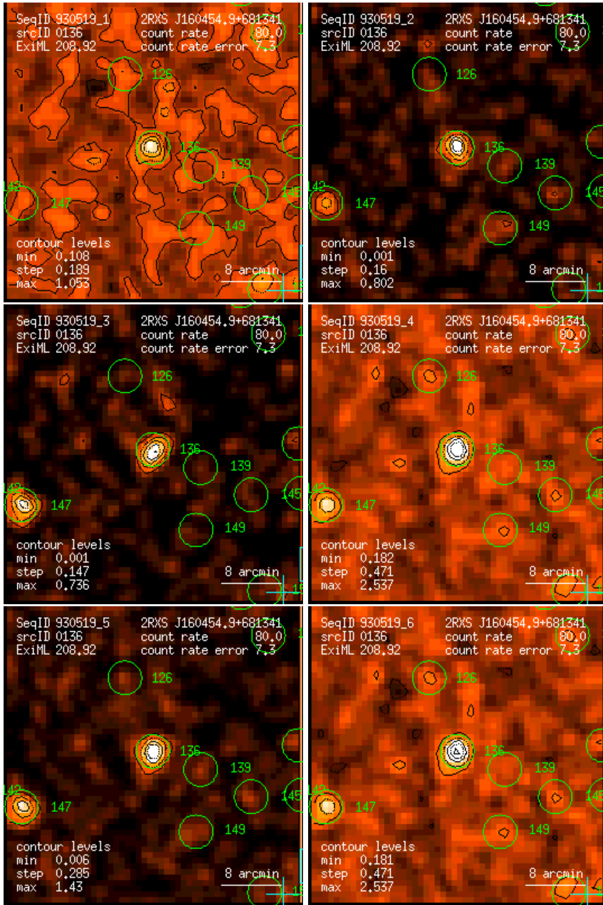
Figure 136: RASS 930519: detection 0136: band rate images, Gaussian filter: (1) PSPC channels 11 – 41, (2) 52 – 90, (3) 91 – 201, (4) 11 – 235, (5) 52 – 201, (6) 11 – 201. Broad band rates in counts/ks. Band rate contour levels in counts/ks/arcmin 2 .
