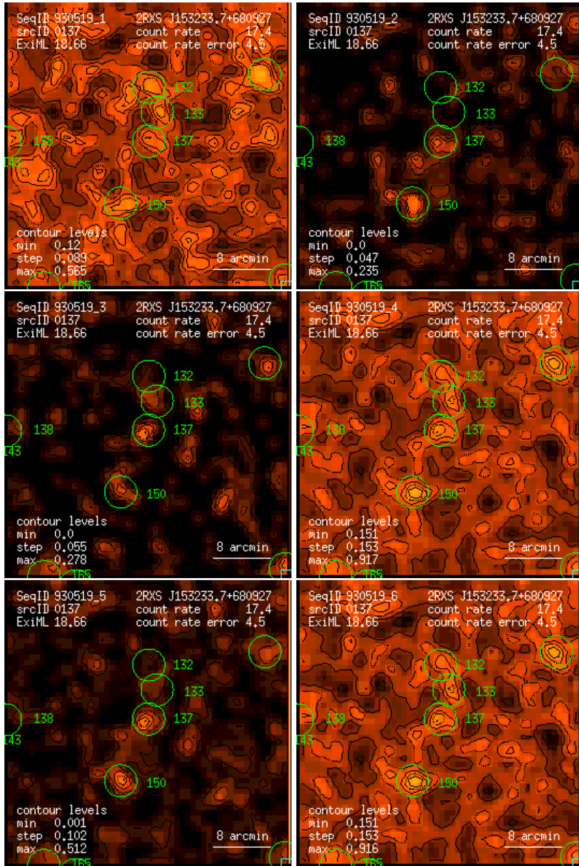
Figure 137: RASS 930519: detection 0137: band rate images, Gaussian filter: (1) PSPC channels 11 – 41, (2) 52 – 90, (3) 91 – 201, (4) 11 – 235, (5) 52 – 201, (6) 11 – 201. Broad band rates in counts/ks. Band rate contour levels in counts/ks/arcmin 2 .
