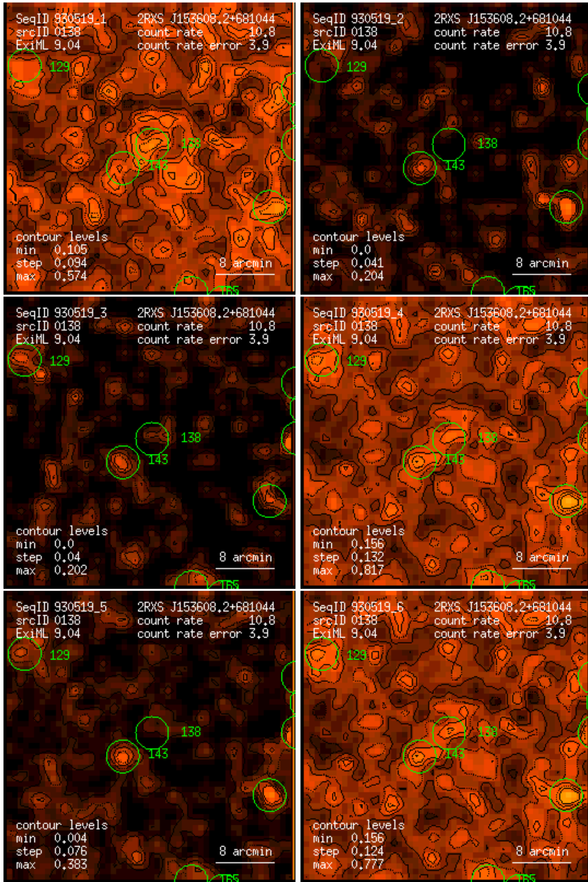
Figure 138: RASS 930519: detection 0138: band rate images, Gaussian filter: (1) PSPC channels 11 – 41, (2) 52 – 90, (3) 91 – 201, (4) 11 – 235, (5) 52 – 201, (6) 11 – 201. Broad band rates in counts/ks. Band rate contour levels in counts/ks/arcmin 2 .
