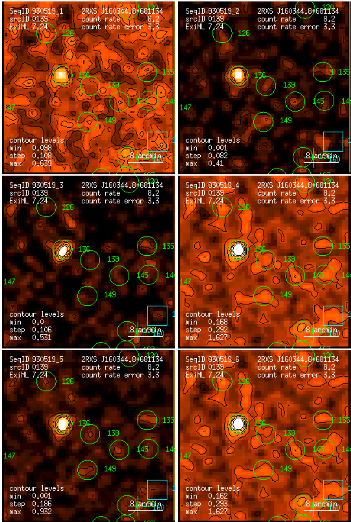
Figure 139: RASS 930519: detection 0139: band rate images, Gaussian filter: (1) PSPC channels 11 – 41, (2) 52 – 90, (3) 91 – 201, (4) 11 – 235, (5) 52 – 201, (6) 11 – 201. Broad band rates in counts/ks. Band rate contour levels in counts/ks/arcmin 2 .
