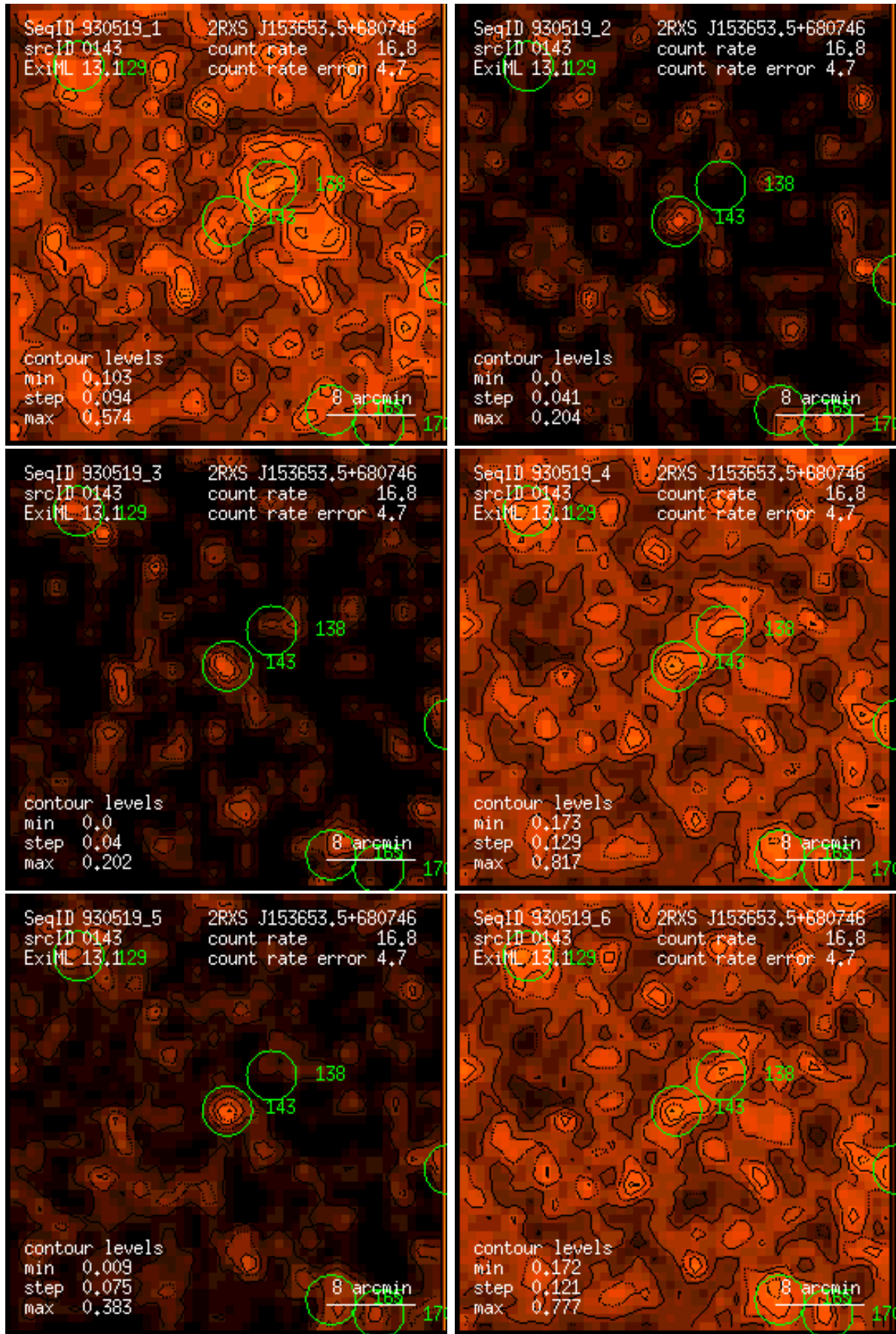
Figure 143: RASS 930519: detection 0143: band rate images, Gaussian filter: (1) PSPC channels 11 – 41, (2) 52 – 90, (3) 91 – 201, (4) 11 – 235, (5) 52 – 201, (6) 11 – 201. Broad band rates in counts/ks. Band rate contour levels in counts/ks/arcmin 2 .
