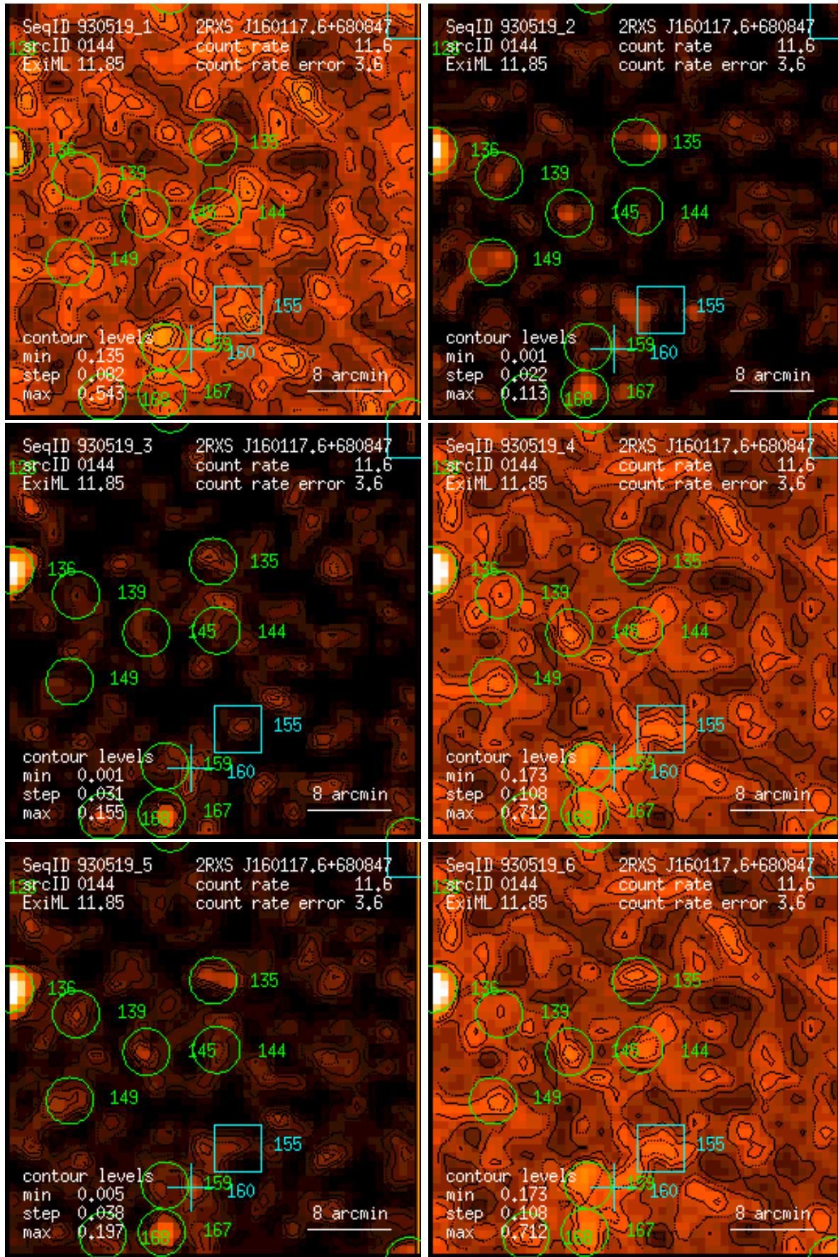
Figure 144: RASS 930519: detection 0144: band rate images, Gaussian filter: (1) PSPC channels 11 – 41, (2) 52 – 90, (3) 91 – 201, (4) 11 – 235, (5) 52 – 201, (6) 11 – 201. Broad band rates in counts/ks. Band rate contour levels in counts/ks/arcmin 2 .
