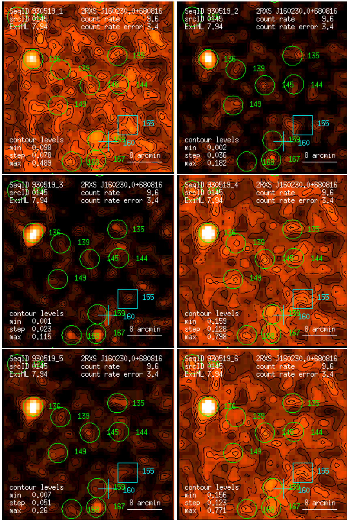
Figure 145: RASS 930519: detection 0145: band rate images, Gaussian filter: (1) PSPC channels 11 – 41, (2) 52 – 90, (3) 91 – 201, (4) 11 – 235, (5) 52 – 201, (6) 11 – 201. Broad band rates in counts/ks. Band rate contour levels in counts/ks/arcmin 2 .
