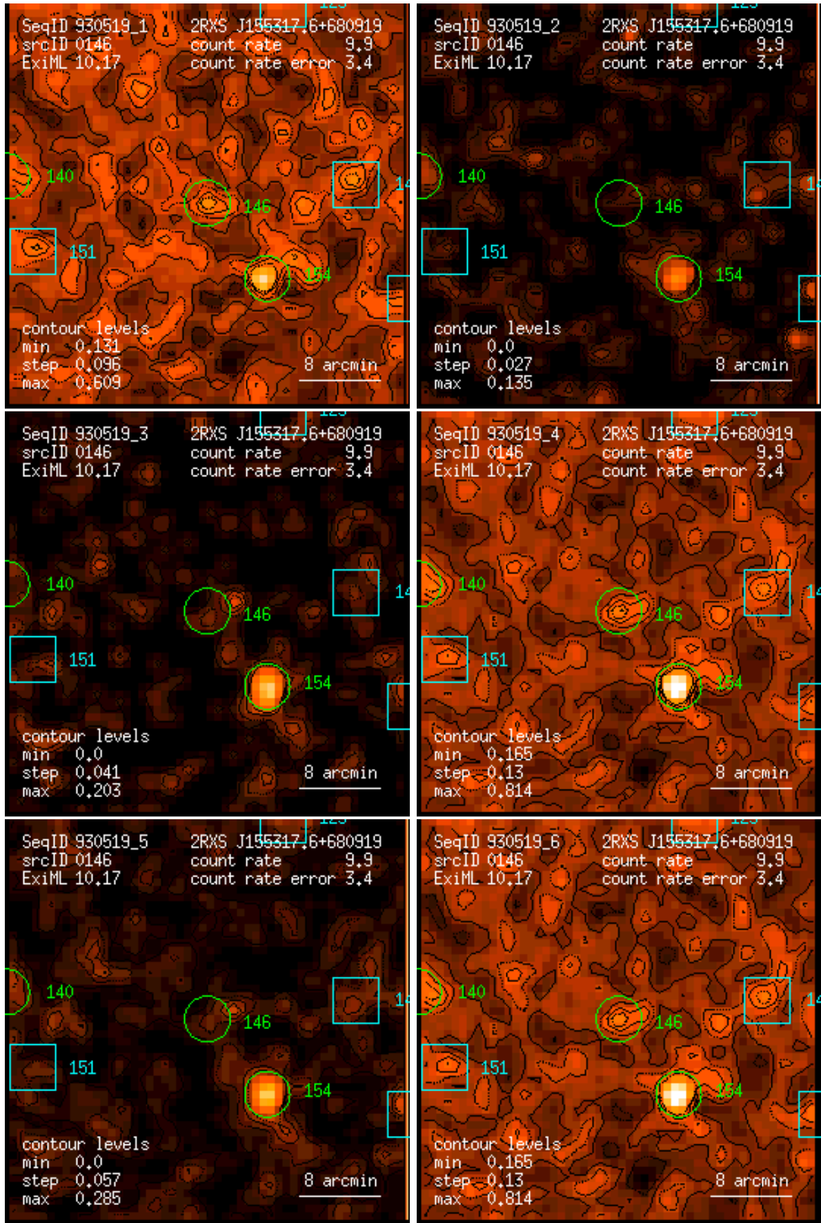
Figure 146: RASS 930519: detection 0146: band rate images, Gaussian filter: (1) PSPC channels 11 – 41, (2) 52 – 90, (3) 91 – 201, (4) 11 – 235, (5) 52 – 201, (6) 11 – 201. Broad band rates in counts/ks. Band rate contour levels in counts/ks/arcmin 2 .
