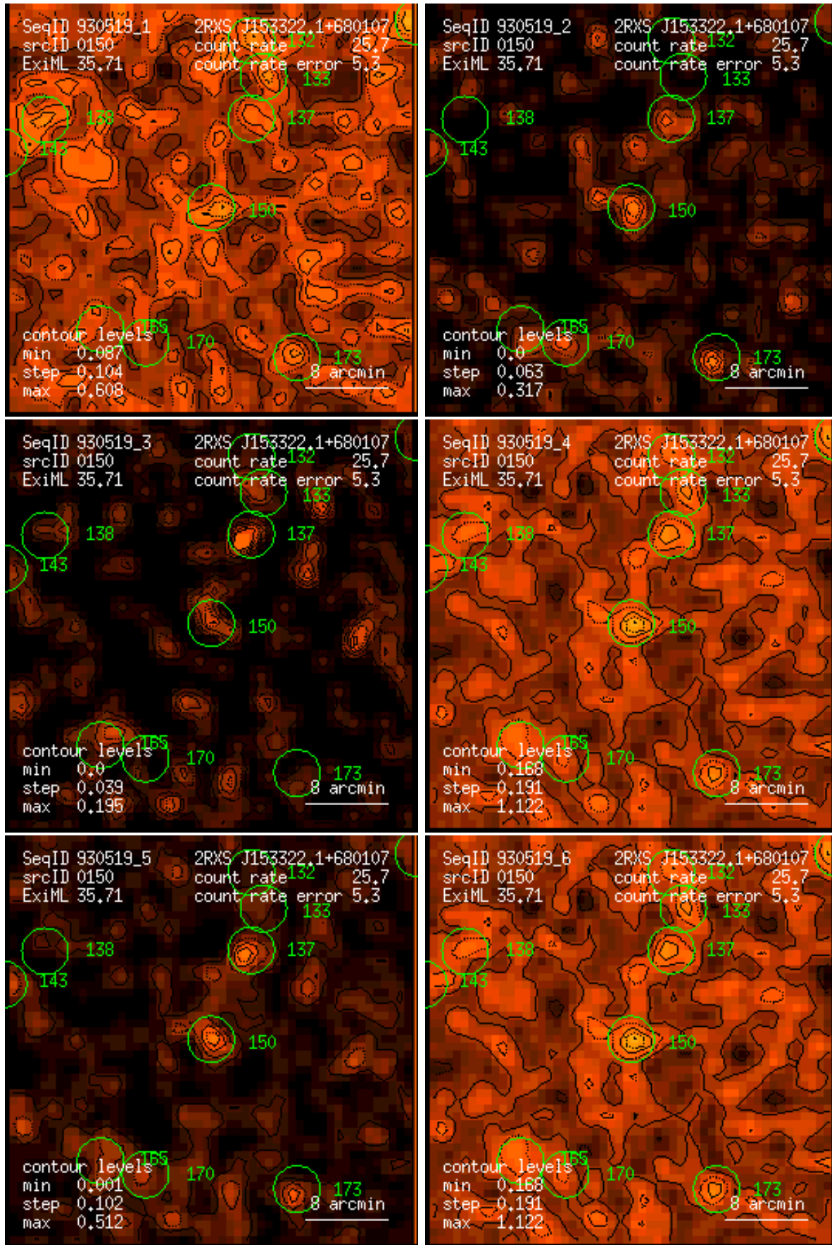
Figure 150: RASS 930519: detection 0150: band rate images, Gaussian filter: (1) PSPC channels 11 – 41, (2) 52 – 90, (3) 91 – 201, (4) 11 – 235, (5) 52 – 201, (6) 11 – 201. Broad band rates in counts/ks. Band rate contour levels in counts/ks/arcmin 2 .
