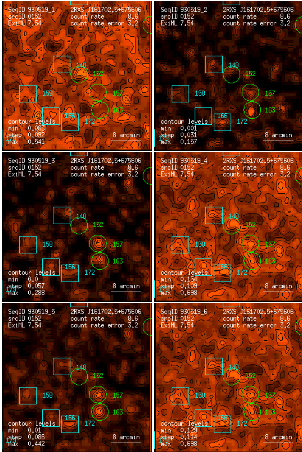
Figure 152: RASS 930519: detection 0152: band rate images, Gaussian filter: (1) PSPC channels 11 – 41, (2) 52 – 90, (3) 91 – 201, (4) 11 – 235, (5) 52 – 201, (6) 11 – 201. Broad band rates in counts/ks. Band rate contour levels in counts/ks/arcmin 2 .
